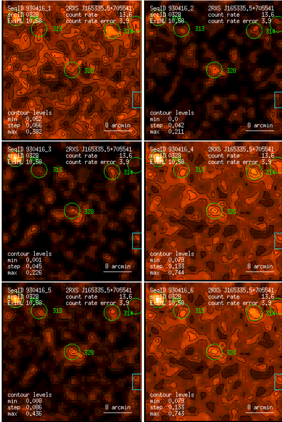
Figure 328: RASS 930416: detection 0328: band rate images, Gaussian filter: (1) PSPC channels 11 – 41, (2) 52 – 90, (3) 91 – 201, (4) 11 – 235, (5) 52 – 201, (6) 11 – 201. Broad band rates in counts/ks. Band rate contour levels in counts/ks/arcmin 2 .
