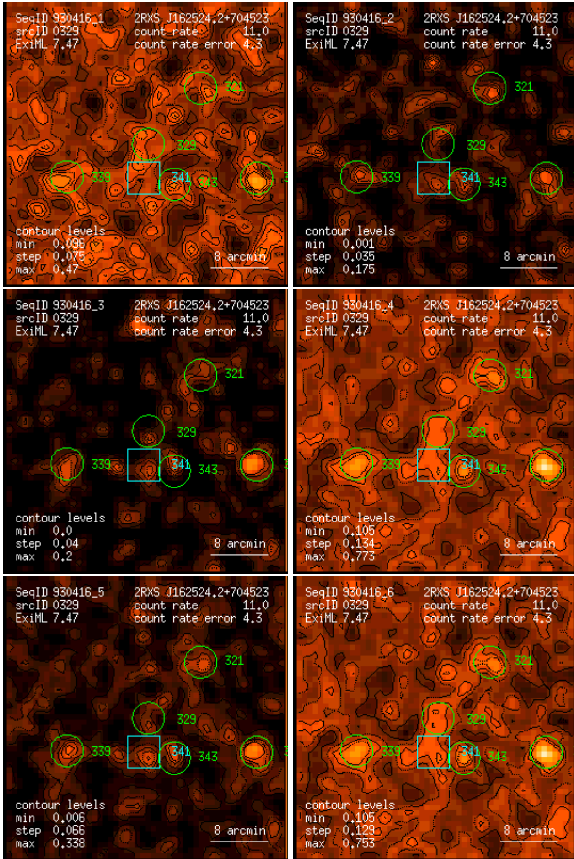
Figure 329: RASS 930416: detection 0329: band rate images, Gaussian filter: (1) PSPC channels 11 – 41, (2) 52 – 90, (3) 91 – 201, (4) 11 – 235, (5) 52 – 201, (6) 11 – 201. Broad band rates in counts/ks. Band rate contour levels in counts/ks/arcmin 2 .
