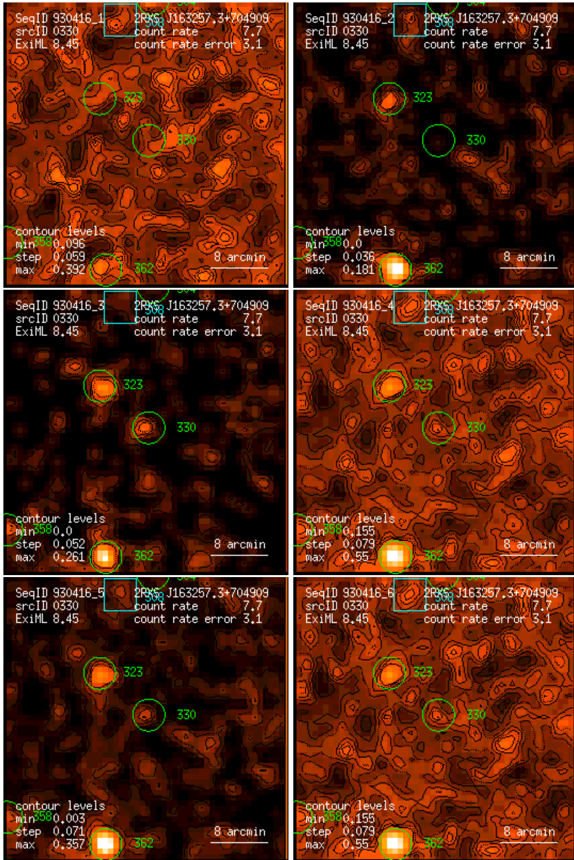
Figure 330: RASS 930416: detection 0330: band rate images, Gaussian filter: (1) PSPC channels 11 – 41, (2) 52 – 90, (3) 91 – 201, (4) 11 – 235, (5) 52 – 201, (6) 11 – 201. Broad band rates in counts/ks. Band rate contour levels in counts/ks/arcmin 2 .
