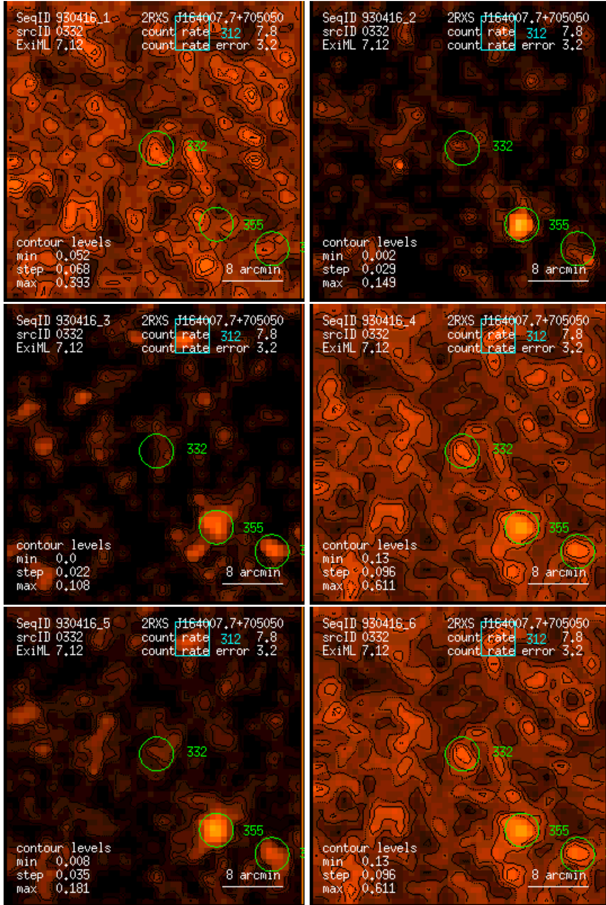
Figure 332: RASS 930416: detection 0332: band rate images, Gaussian filter: (1) PSPC channels 11 – 41, (2) 52 – 90, (3) 91 – 201, (4) 11 – 235, (5) 52 – 201, (6) 11 – 201. Broad band rates in counts/ks. Band rate contour levels in counts/ks/arcmin 2 .
