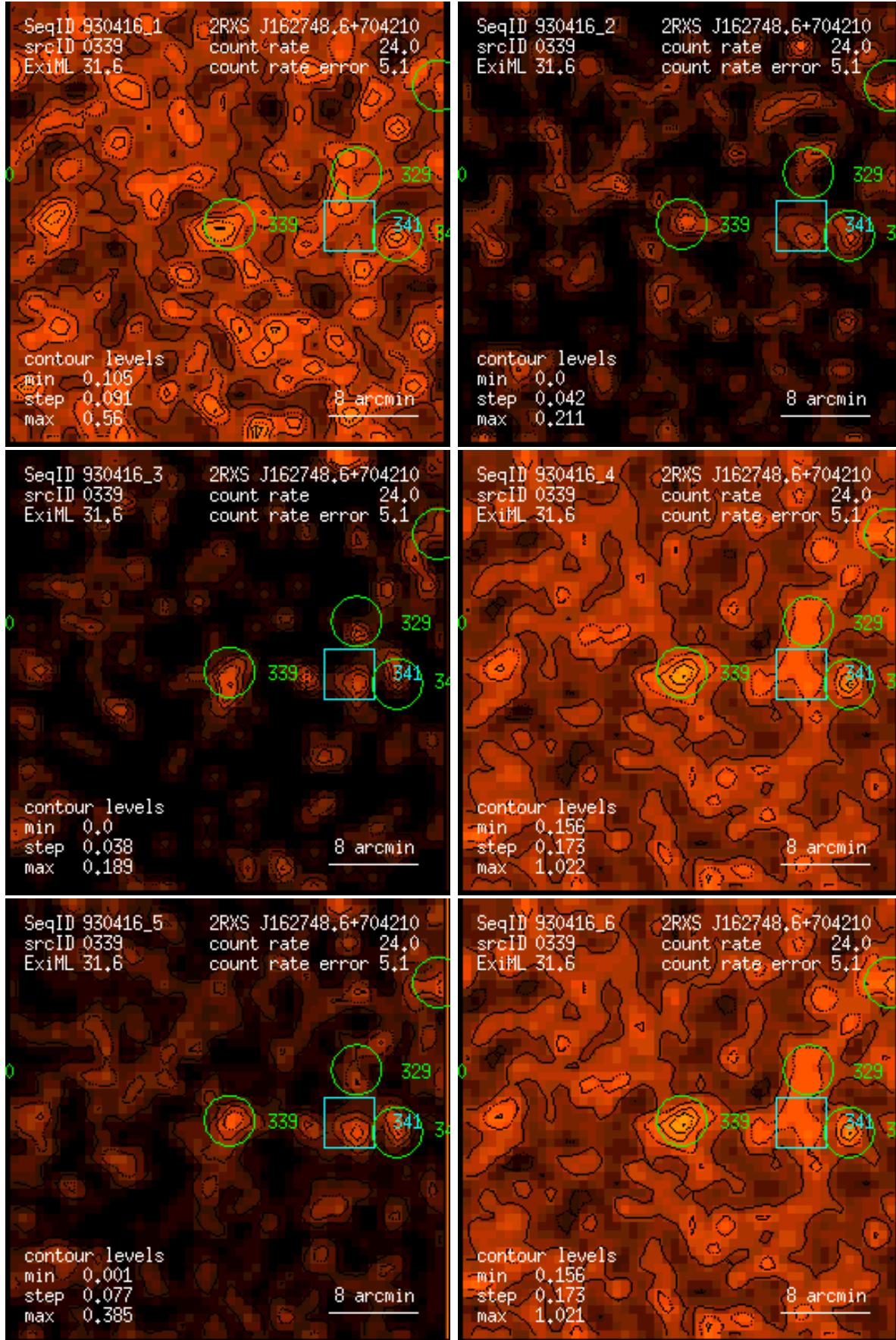
Figure 339: RASS 930416: detection 0339: band rate images, Gaussian filter: (1) PSPC channels 11 – 41, (2) 52 – 90, (3) 91 – 201, (4) 11 – 235, (5) 52 – 201, (6) 11 – 201. Broad band rates in counts/ks. Band rate contour levels in counts/ks/arcmin 2 .
