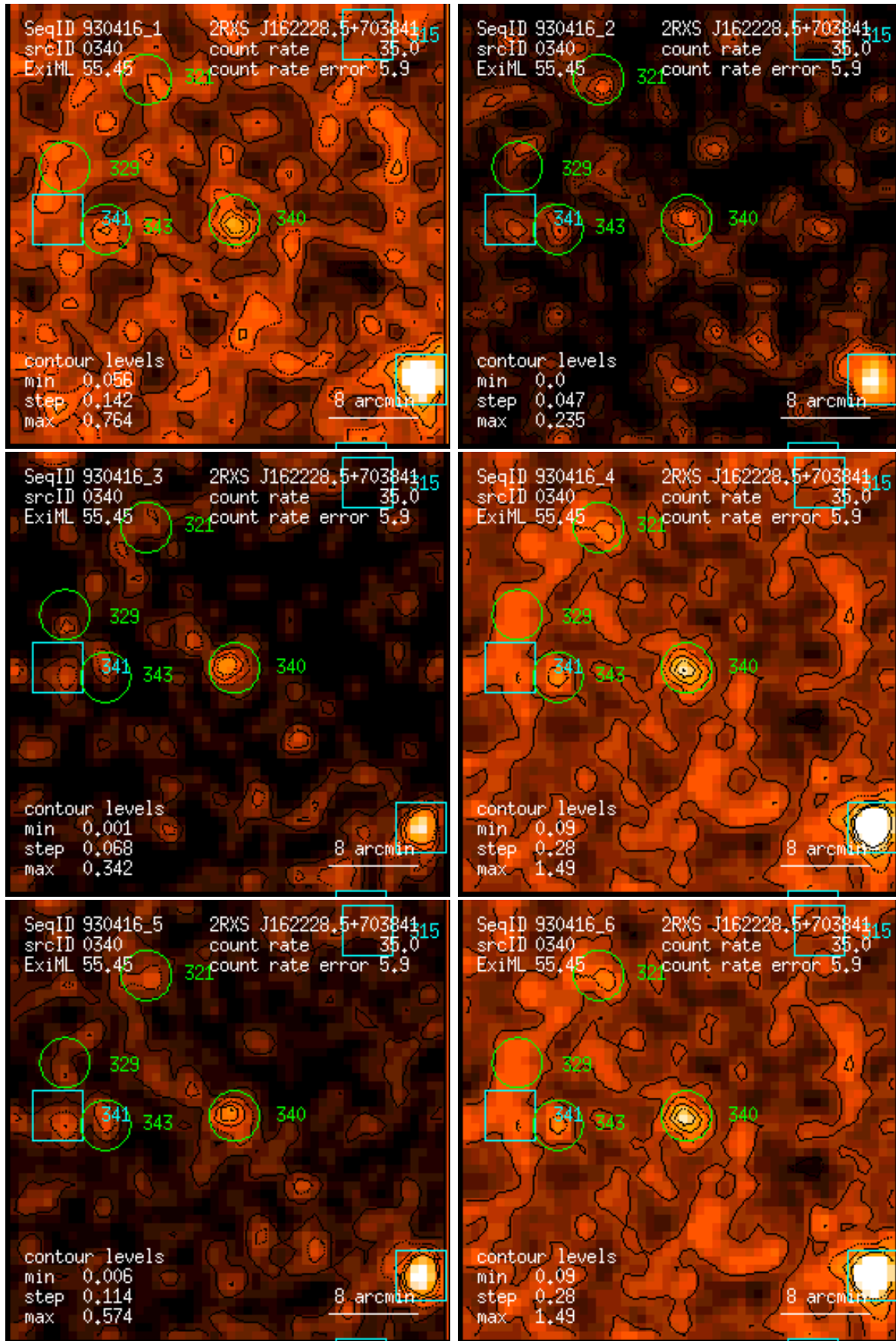
Figure 340: RASS 930416: detection 0340: band rate images, Gaussian filter: (1) PSPC channels 11 – 41, (2) 52 – 90, (3) 91 – 201, (4) 11 – 235, (5) 52 – 201, (6) 11 – 201. Broad band rates in counts/ks. Band rate contour levels in counts/ks/arcmin 2 .
