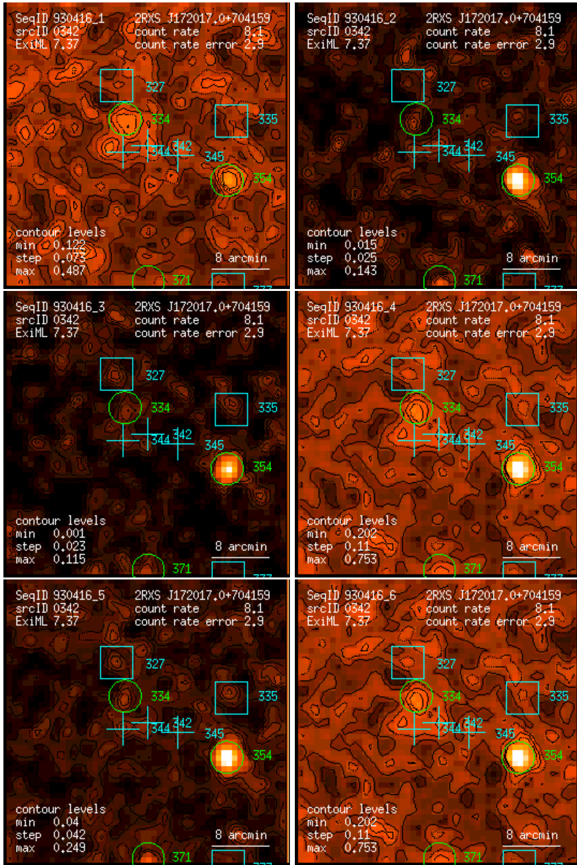
Figure 342: RASS 930416: detection 0342: band rate images, Gaussian filter: (1) PSPC channels 11 – 41, (2) 52 – 90, (3) 91 – 201, (4) 11 – 235, (5) 52 – 201, (6) 11 – 201. Broad band rates in counts/ks. Band rate contour levels in counts/ks/arcmin 2 .
