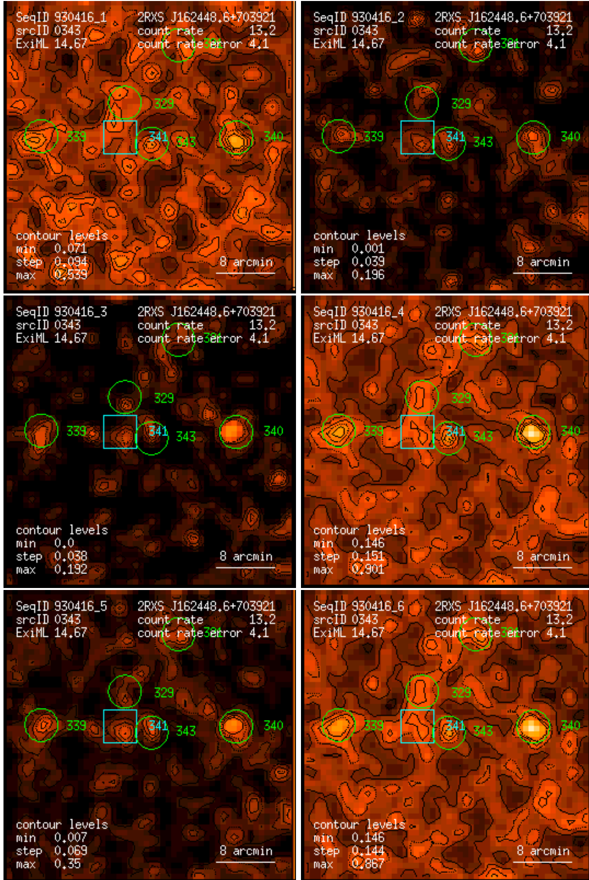
Figure 343: RASS 930416: detection 0343: band rate images, Gaussian filter: (1) PSPC channels 11 – 41, (2) 52 – 90, (3) 91 – 201, (4) 11 – 235, (5) 52 – 201, (6) 11 – 201. Broad band rates in counts/ks. Band rate contour levels in counts/ks/arcmin 2 .
