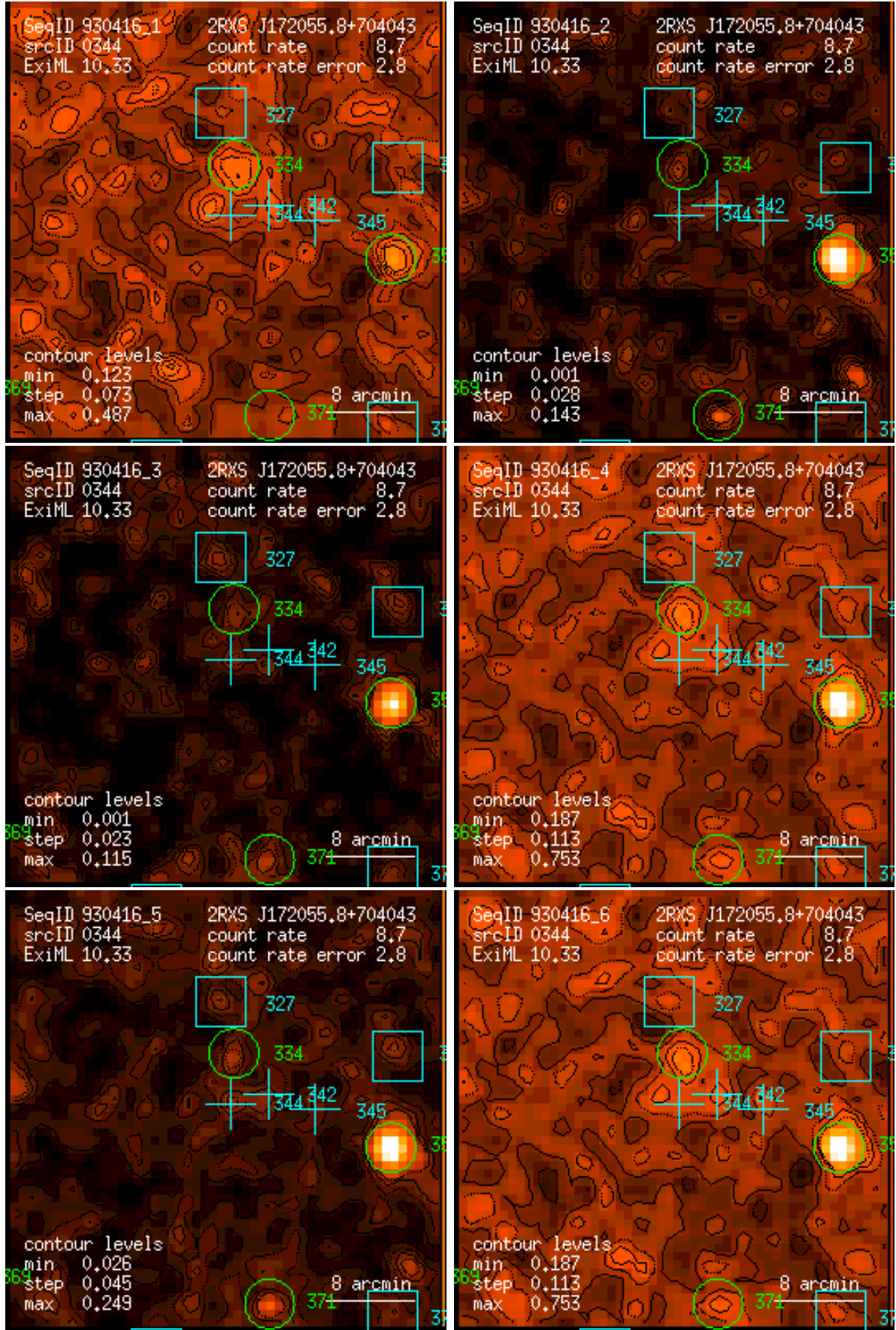
Figure 344: RASS 930416: detection 0344: band rate images, Gaussian filter: (1) PSPC channels 11 – 41, (2) 52 – 90, (3) 91 – 201, (4) 11 – 235, (5) 52 – 201, (6) 11 – 201. Broad band rates in counts/ks. Band rate contour levels in counts/ks/arcmin 2 .
