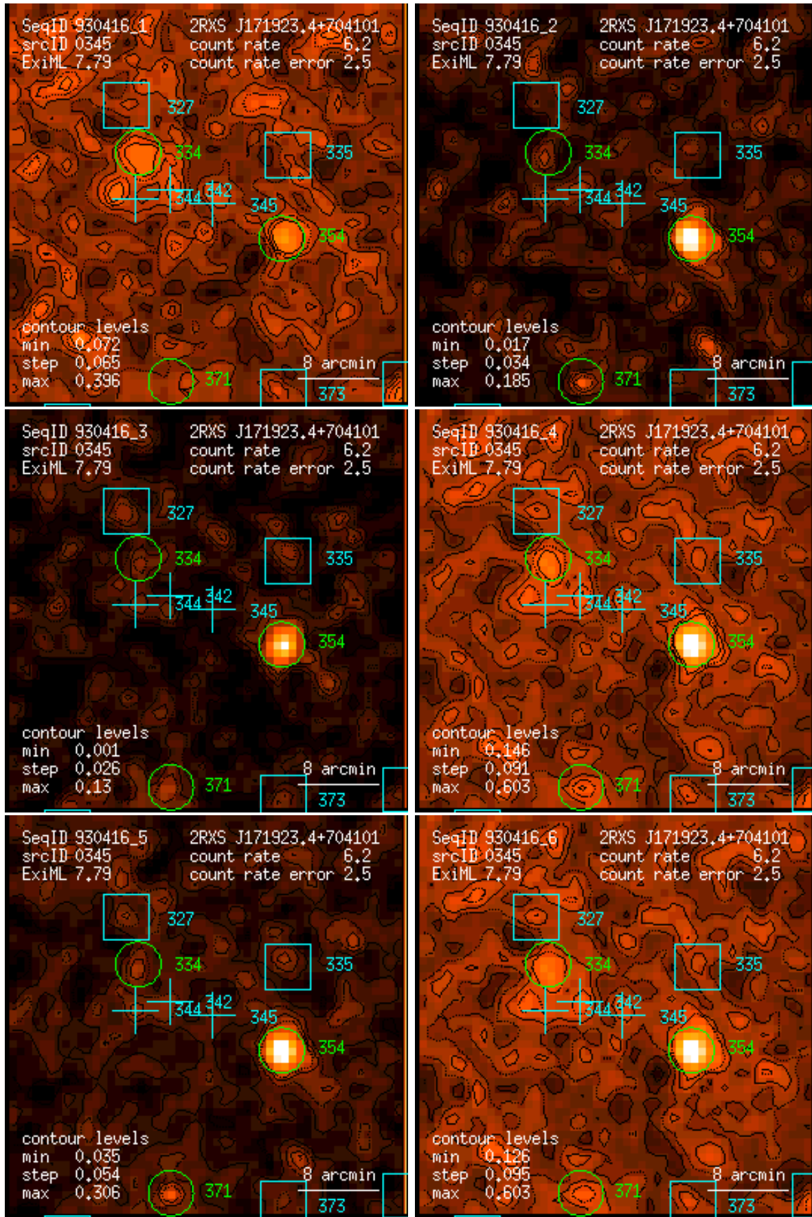
Figure 345: RASS 930416: detection 0345: band rate images, Gaussian filter: (1) PSPC channels 11 – 41, (2) 52 – 90, (3) 91 – 201, (4) 11 – 235, (5) 52 – 201, (6) 11 – 201. Broad band rates in counts/ks. Band rate contour levels in counts/ks/arcmin 2 .
