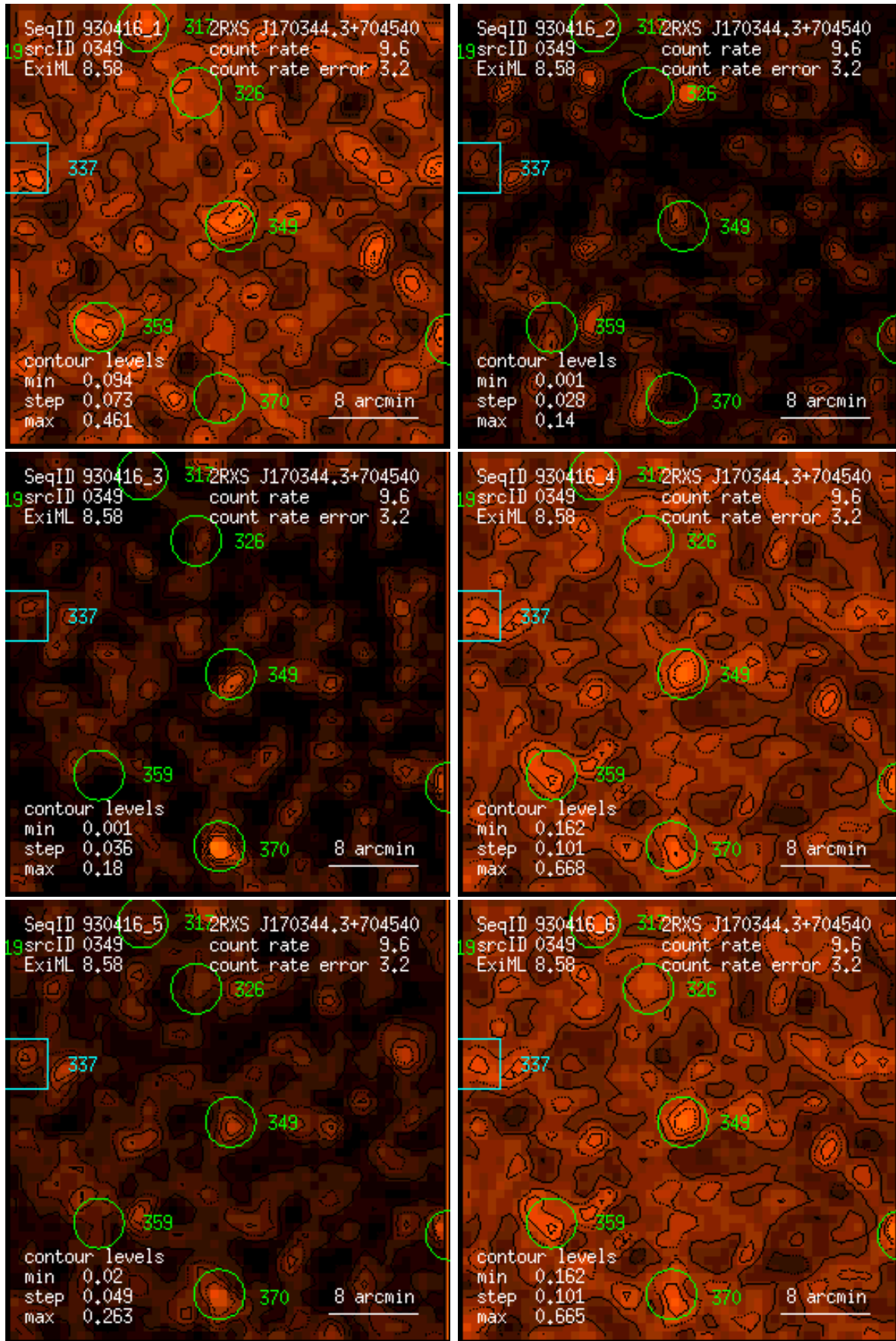
Figure 349: RASS 930416: detection 0349: band rate images, Gaussian filter: (1) PSPC channels 11 – 41, (2) 52 – 90, (3) 91 – 201, (4) 11 – 235, (5) 52 – 201, (6) 11 – 201. Broad band rates in counts/ks. Band rate contour levels in counts/ks/arcmin 2 .
