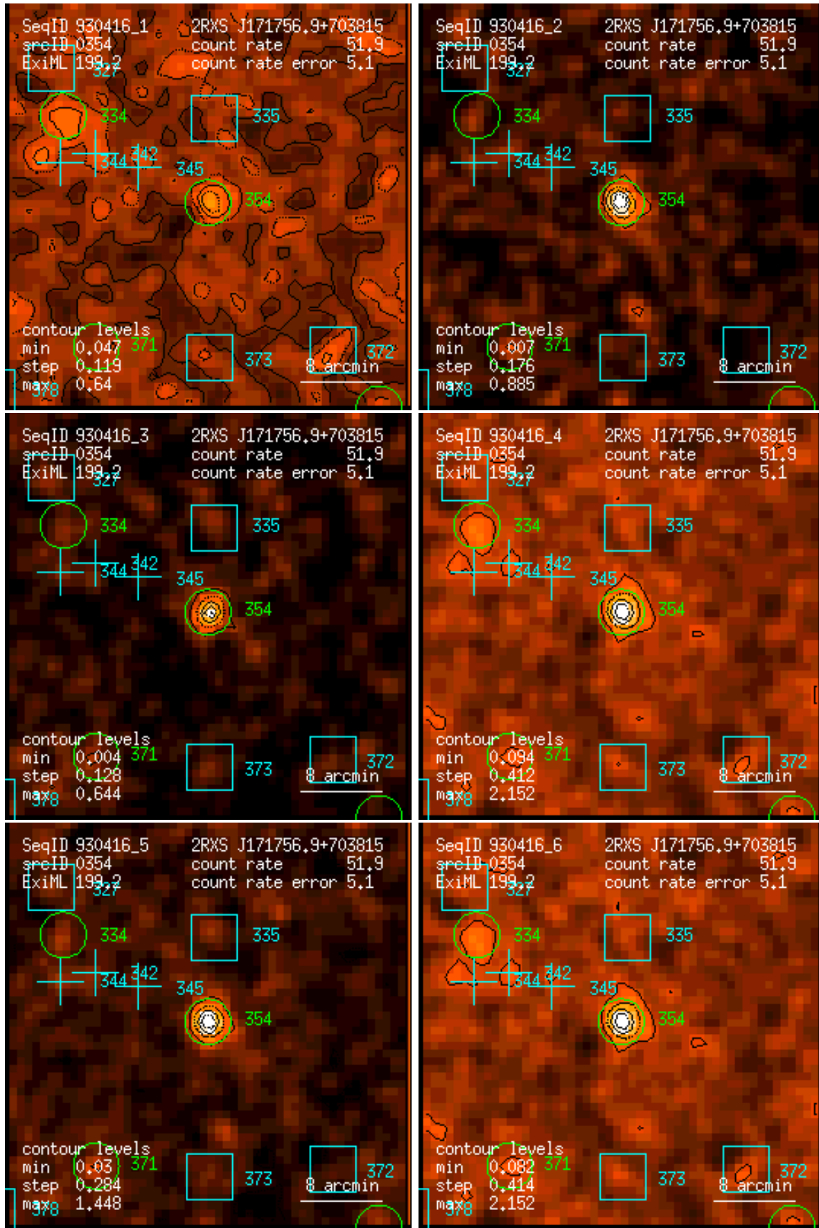
Figure 354: RASS 930416: detection 0354: band rate images, Gaussian filter: (1) PSPC channels 11 – 41, (2) 52 – 90, (3) 91 – 201, (4) 11 – 235, (5) 52 – 201, (6) 11 – 201. Broad band rates in counts/ks. Band rate contour levels in counts/ks/arcmin 2 .
