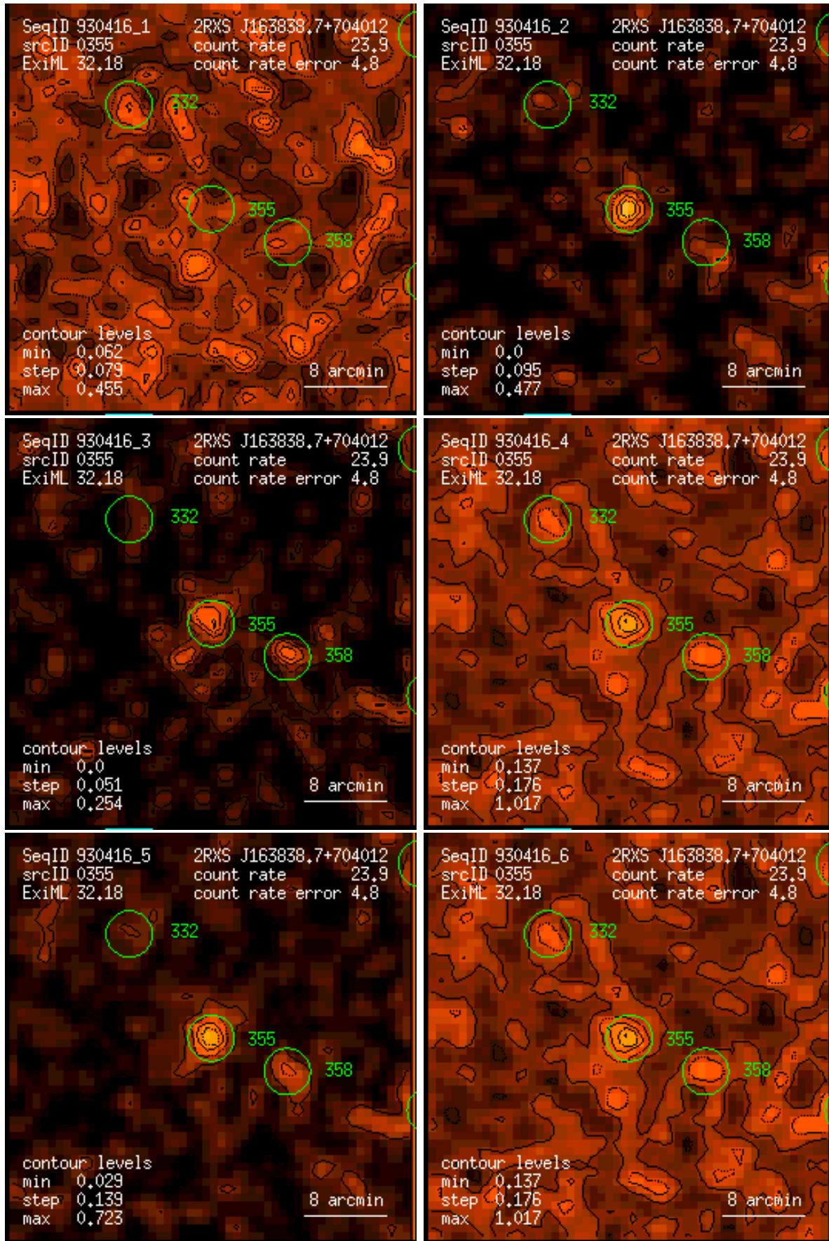
Figure 355: RASS 930416: detection 0355: band rate images, Gaussian filter: (1) PSPC channels 11 – 41, (2) 52 – 90, (3) 91 – 201, (4) 11 – 235, (5) 52 – 201, (6) 11 – 201. Broad band rates in counts/ks. Band rate contour levels in counts/ks/arcmin 2 .
