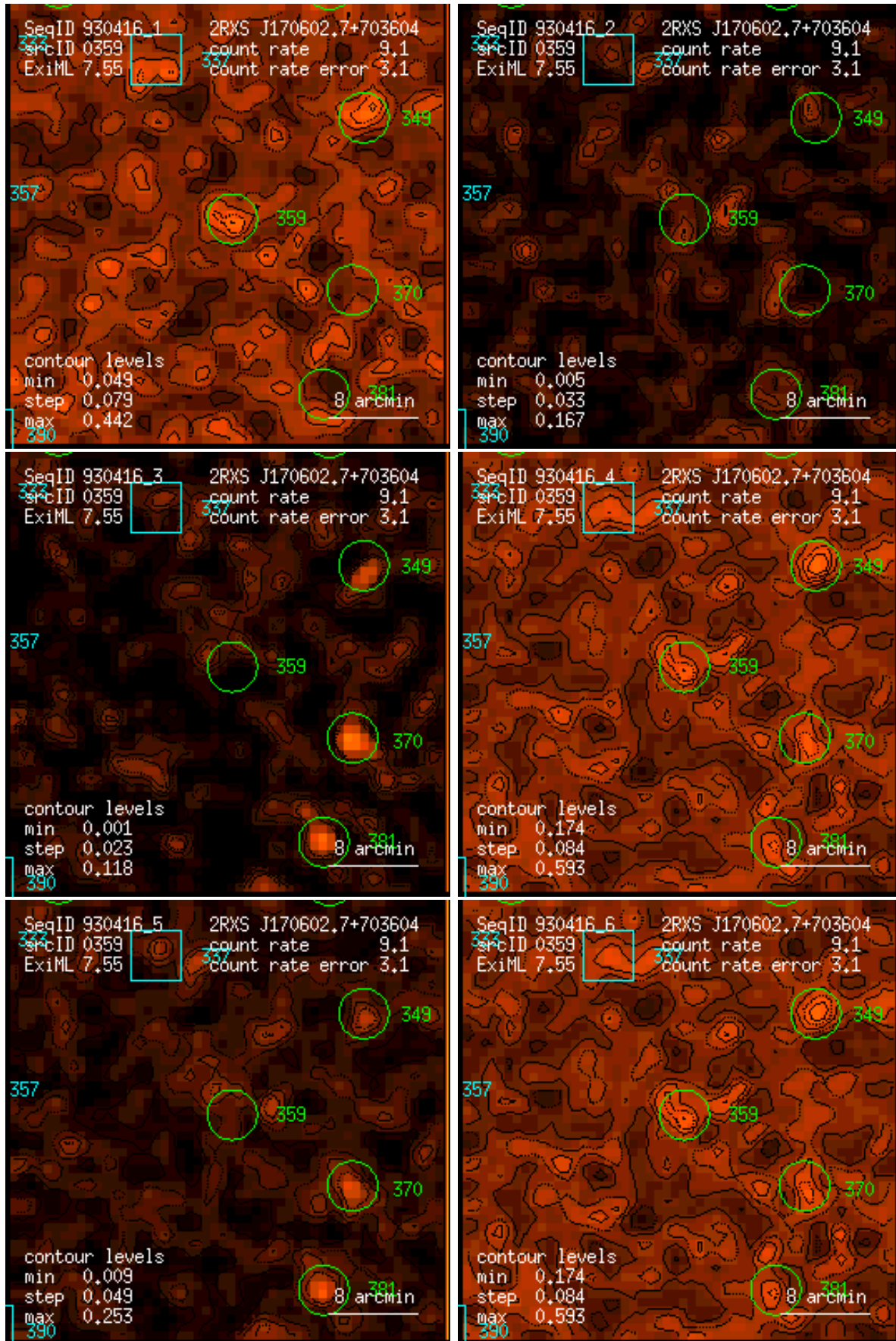
Figure 359: RASS 930416: detection 0359: band rate images, Gaussian filter: (1) PSPC channels 11 – 41, (2) 52 – 90, (3) 91 – 201, (4) 11 – 235, (5) 52 – 201, (6) 11 – 201. Broad band rates in counts/ks. Band rate contour levels in counts/ks/arcmin 2 .
