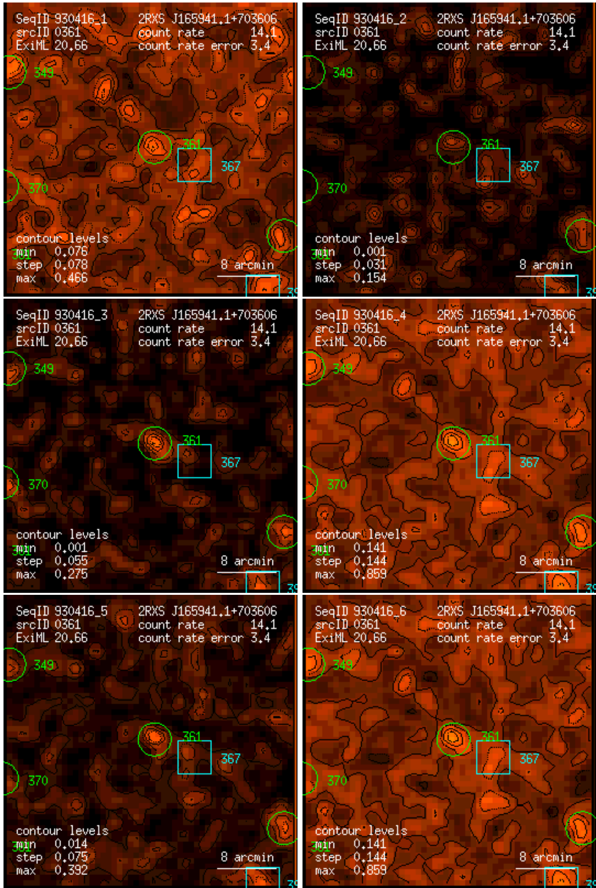
Figure 361: RASS 930416: detection 0361: band rate images, Gaussian filter: (1) PSPC channels 11 – 41, (2) 52 – 90, (3) 91 – 201, (4) 11 – 235, (5) 52 – 201, (6) 11 – 201. Broad band rates in counts/ks. Band rate contour levels in counts/ks/arcmin 2 .
