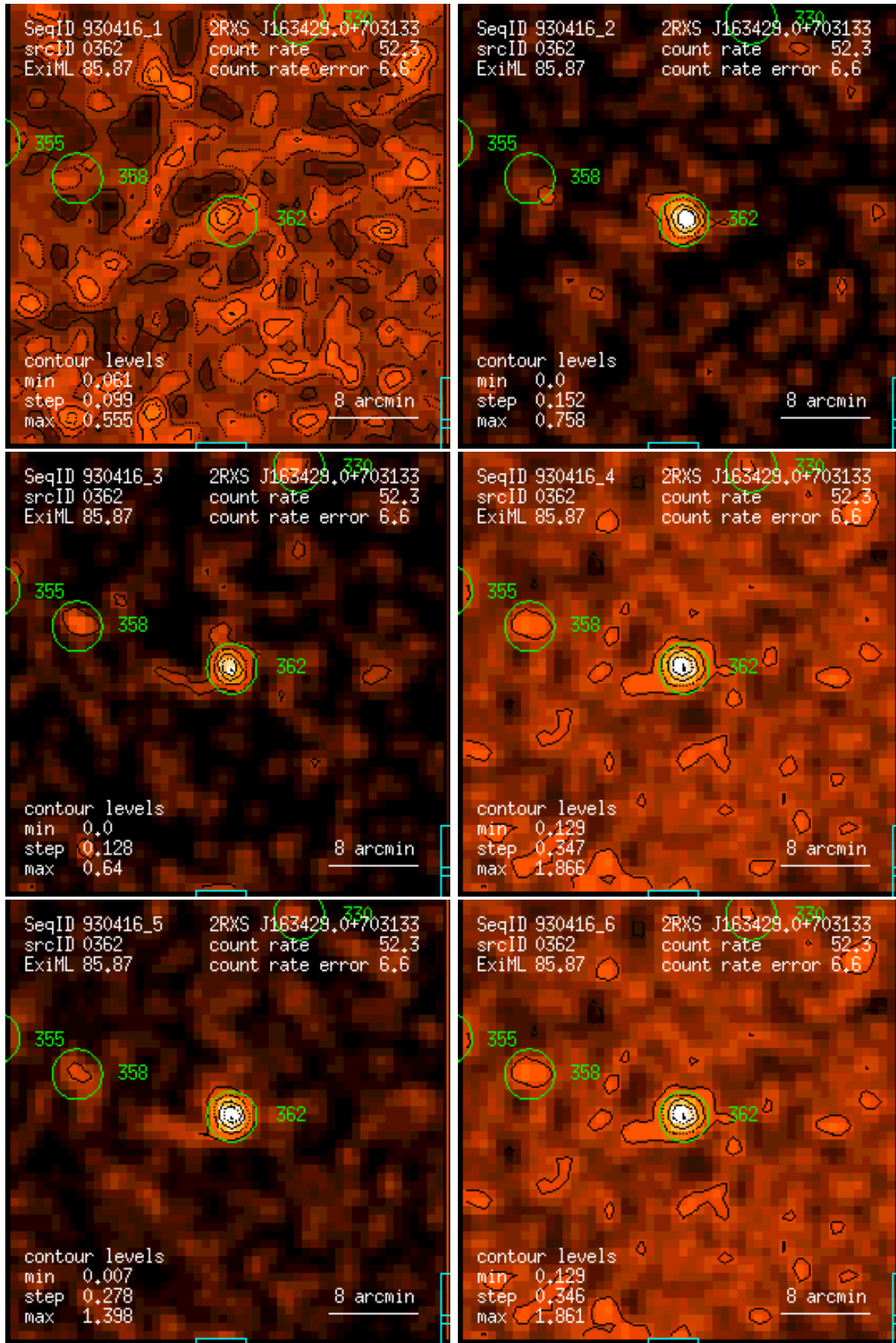
Figure 362: RASS 930416: detection 0362: band rate images, Gaussian filter: (1) PSPC channels 11 – 41, (2) 52 – 90, (3) 91 – 201, (4) 11 – 235, (5) 52 – 201, (6) 11 – 201. Broad band rates in counts/ks. Band rate contour levels in counts/ks/arcmin 2 .
