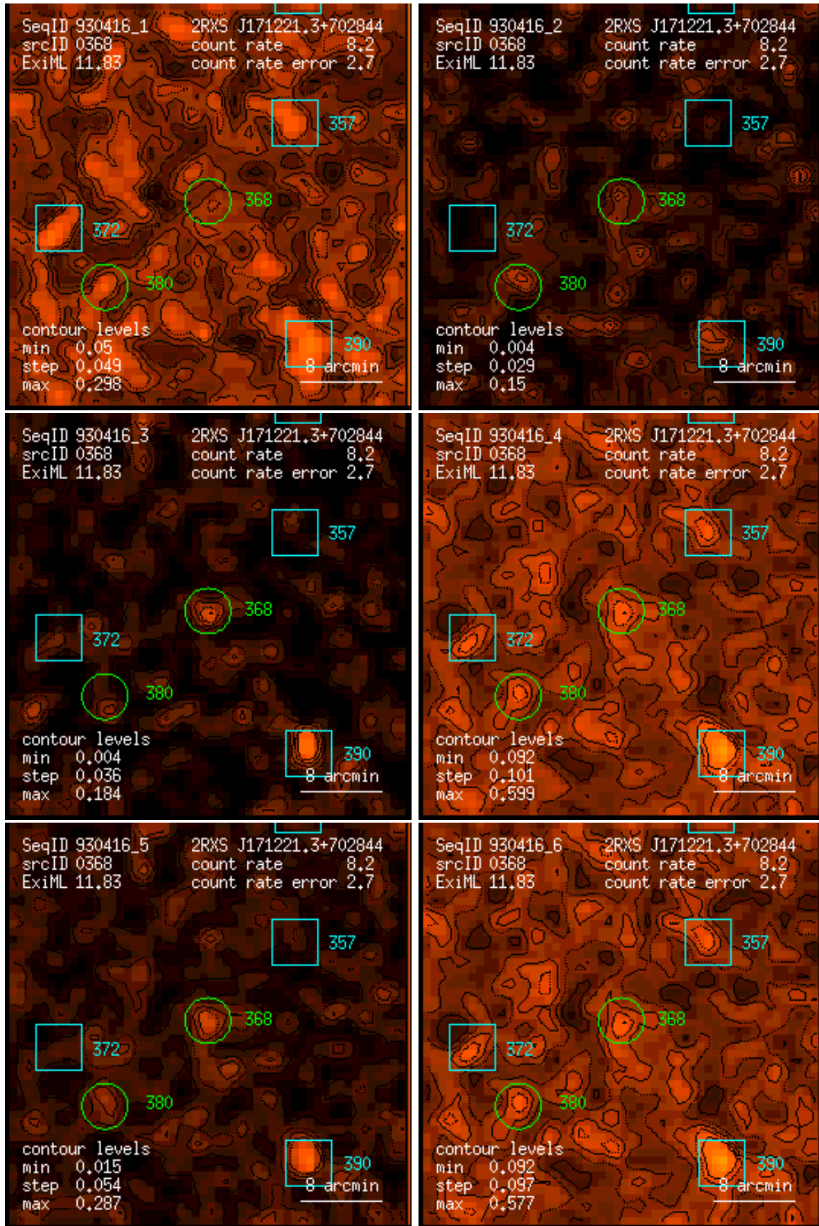
Figure 368: RASS 930416: detection 0368: band rate images, Gaussian filter: (1) PSPC channels 11 – 41, (2) 52 – 90, (3) 91 – 201, (4) 11 – 235, (5) 52 – 201, (6) 11 – 201. Broad band rates in counts/ks. Band rate contour levels in counts/ks/arcmin 2 .
