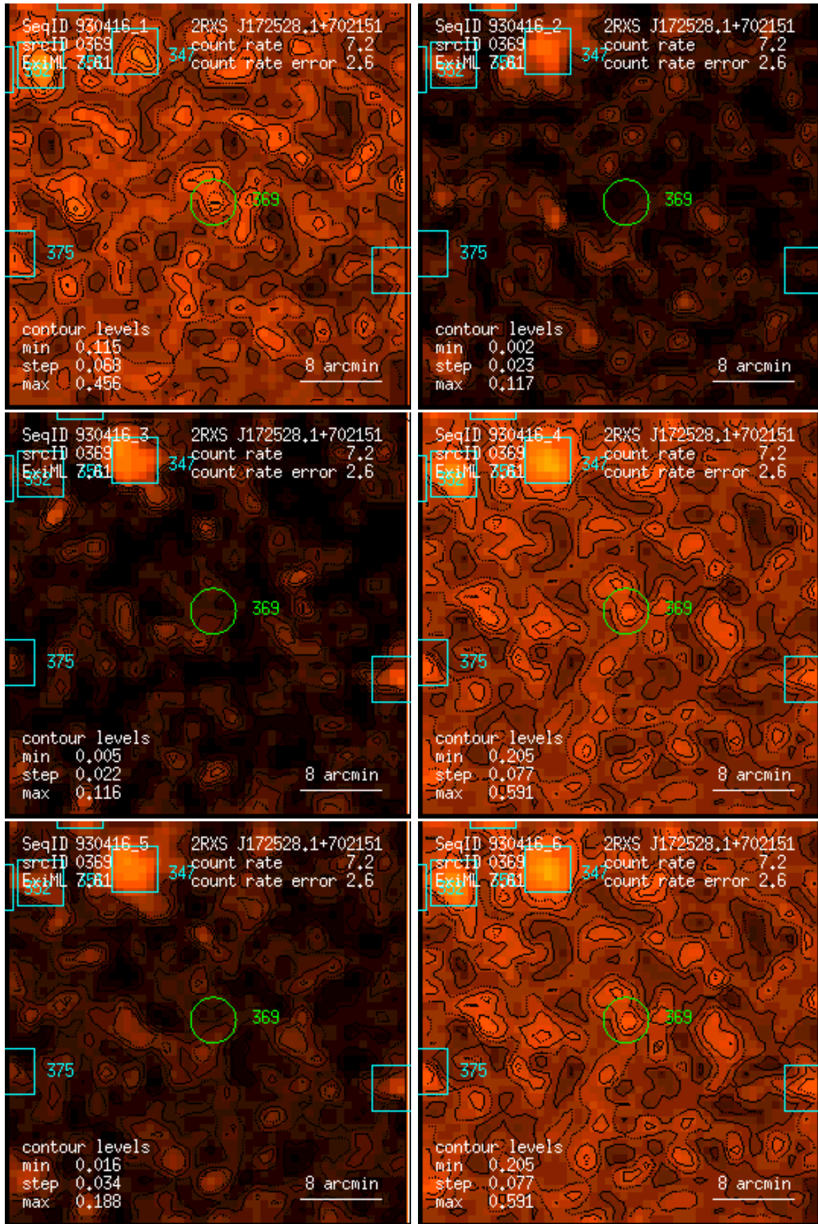
Figure 369: RASS 930416: detection 0369: band rate images, Gaussian filter: (1) PSPC channels 11 – 41, (2) 52 – 90, (3) 91 – 201, (4) 11 – 235, (5) 52 – 201, (6) 11 – 201. Broad band rates in counts/ks. Band rate contour levels in counts/ks/arcmin 2 .
