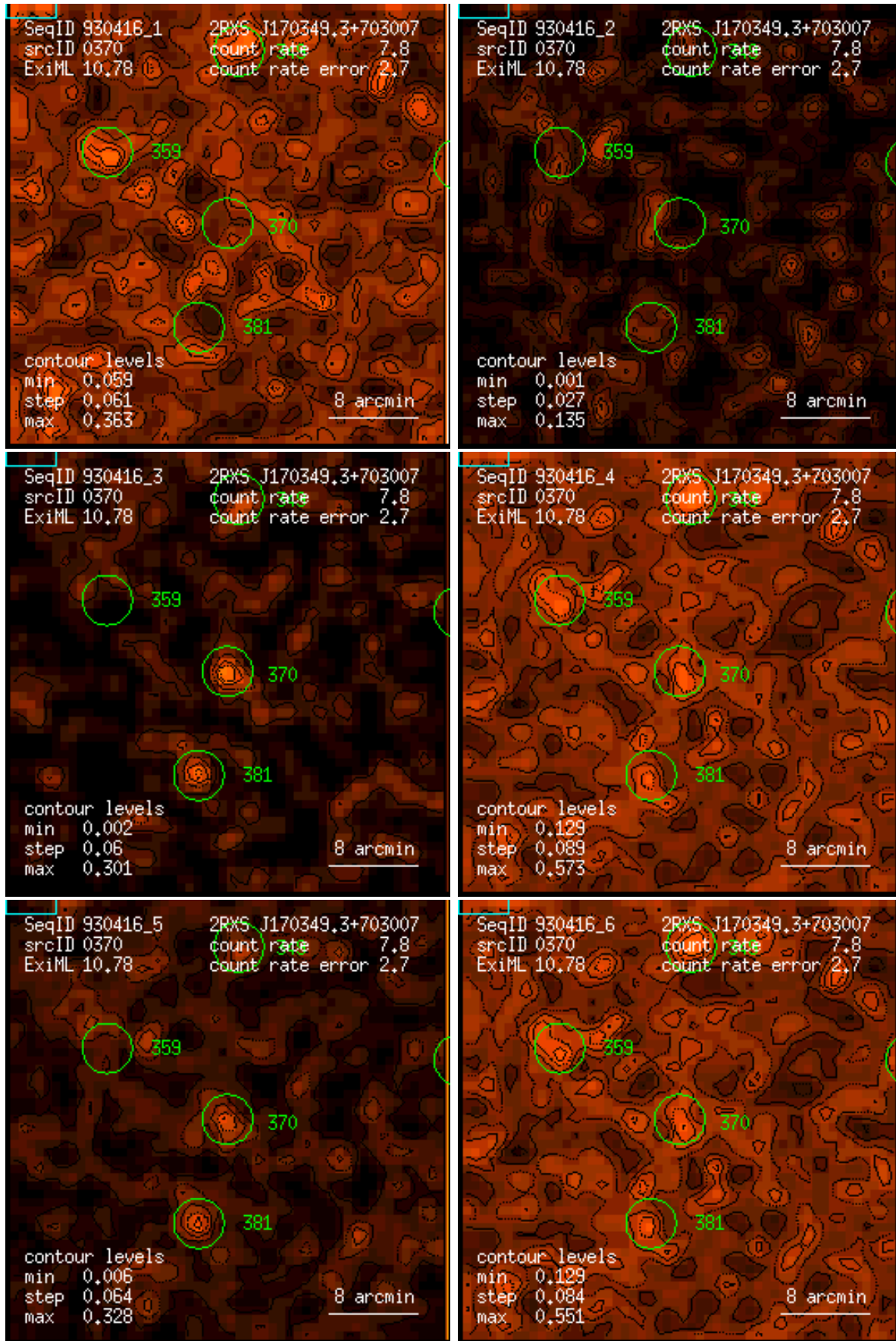
Figure 370: RASS 930416: detection 0370: band rate images, Gaussian filter: (1) PSPC channels 11 – 41, (2) 52 – 90, (3) 91 – 201, (4) 11 – 235, (5) 52 – 201, (6) 11 – 201. Broad band rates in counts/ks. Band rate contour levels in counts/ks/arcmin 2 .
