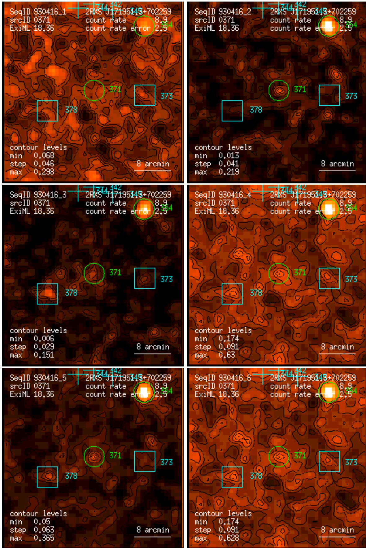
Figure 371: RASS 930416: detection 0371: band rate images, Gaussian filter: (1) PSPC channels 11 – 41, (2) 52 – 90, (3) 91 – 201, (4) 11 – 235, (5) 52 – 201, (6) 11 – 201. Broad band rates in counts/ks. Band rate contour levels in counts/ks/arcmin 2 .
