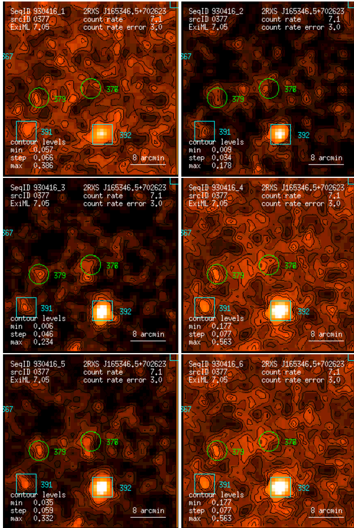
Figure 377: RASS 930416: detection 0377: band rate images, Gaussian filter: (1) PSPC channels 11 – 41, (2) 52 – 90, (3) 91 – 201, (4) 11 – 235, (5) 52 – 201, (6) 11 – 201. Broad band rates in counts/ks. Band rate contour levels in counts/ks/arcmin 2 .
