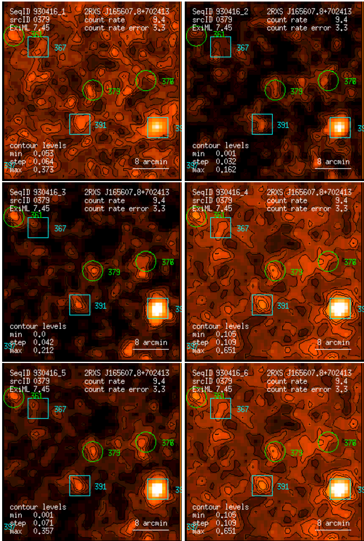
Figure 379: RASS 930416: detection 0379: band rate images, Gaussian filter: (1) PSPC channels 11 – 41, (2) 52 – 90, (3) 91 – 201, (4) 11 – 235, (5) 52 – 201, (6) 11 – 201. Broad band rates in counts/ks. Band rate contour levels in counts/ks/arcmin 2 .
