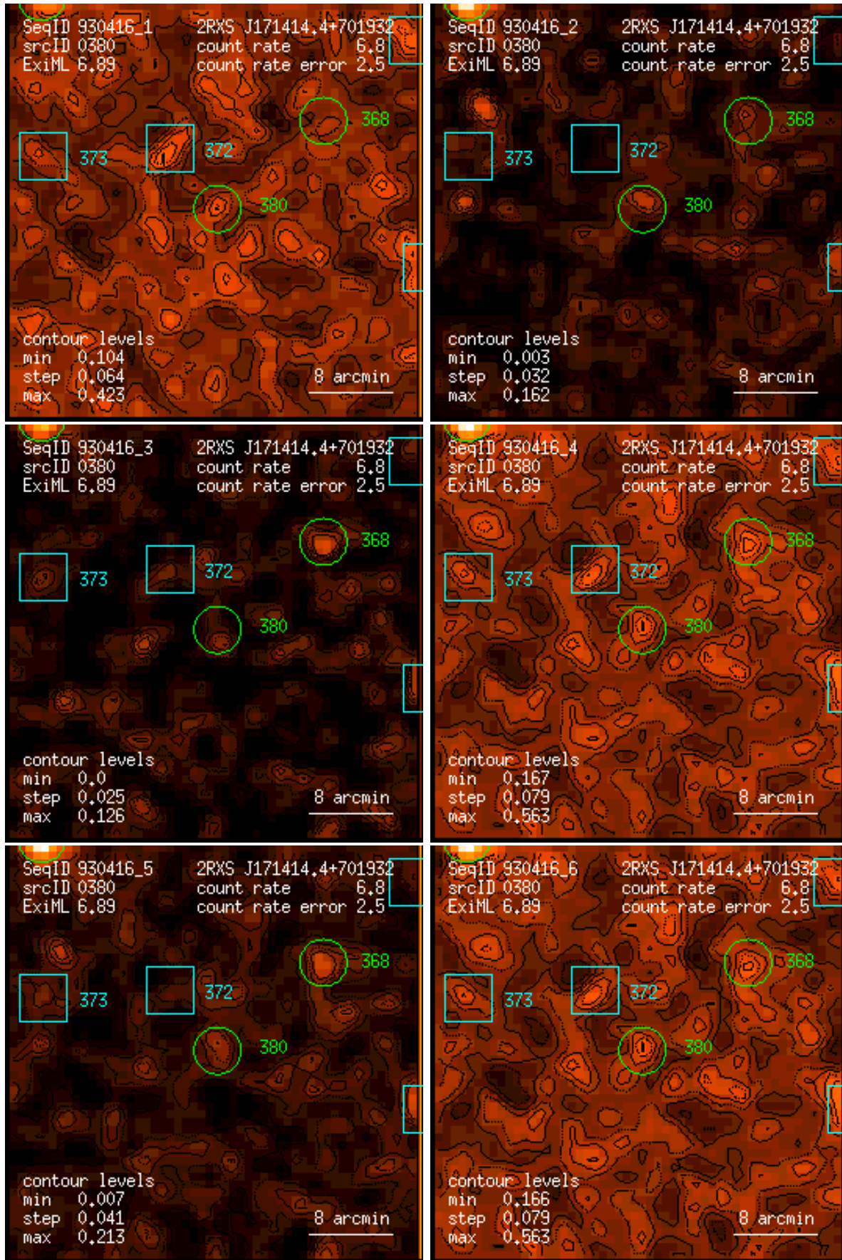
Figure 380: RASS 930416: detection 0380: band rate images, Gaussian filter: (1) PSPC channels 11 – 41, (2) 52 – 90, (3) 91 – 201, (4) 11 – 235, (5) 52 – 201, (6) 11 – 201. Broad band rates in counts/ks. Band rate contour levels in counts/ks/arcmin 2 .
