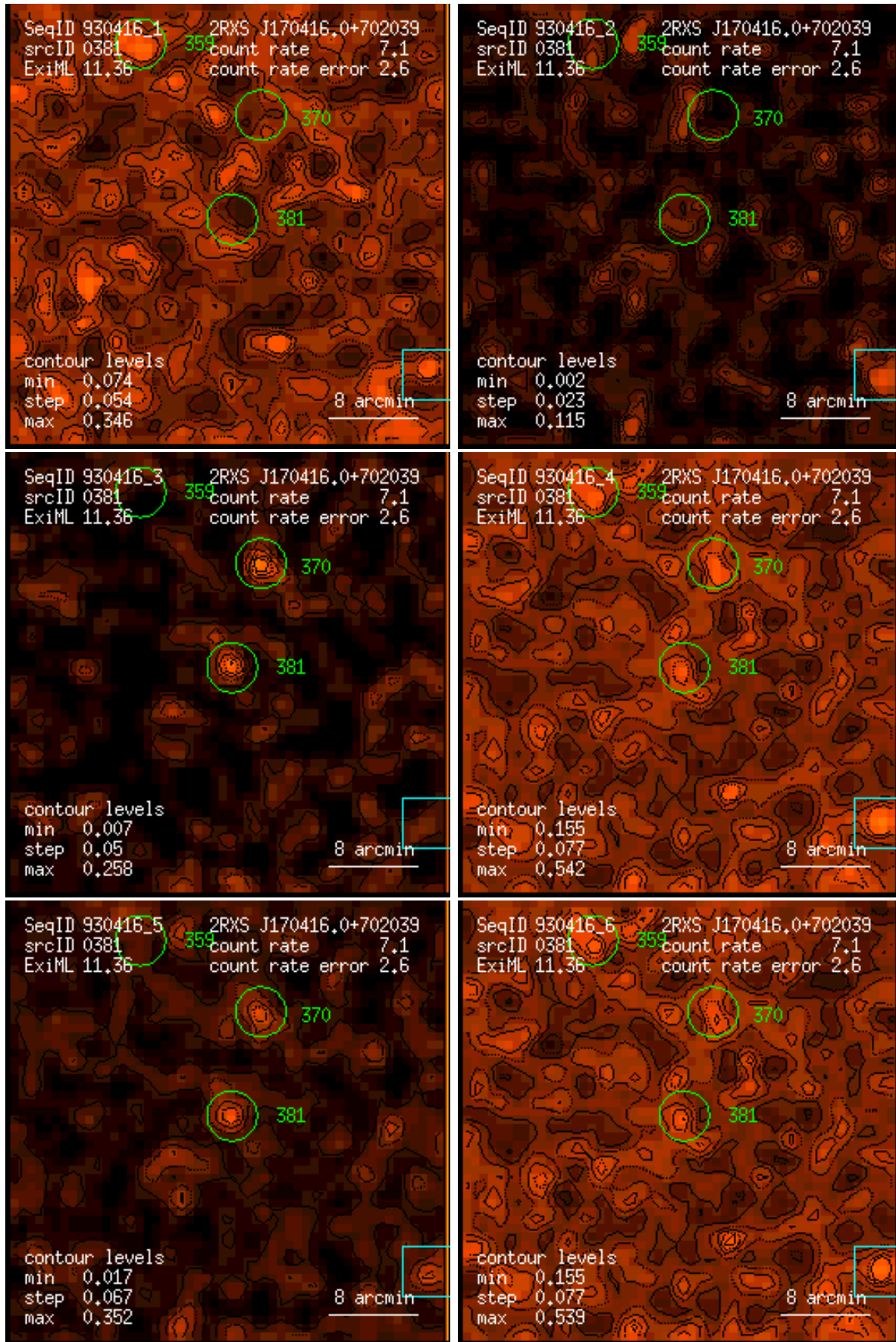
Figure 381: RASS 930416: detection 0381: band rate images, Gaussian filter: (1) PSPC channels 11 – 41, (2) 52 – 90, (3) 91 – 201, (4) 11 – 235, (5) 52 – 201, (6) 11 – 201. Broad band rates in counts/ks. Band rate contour levels in counts/ks/arcmin 2 .
