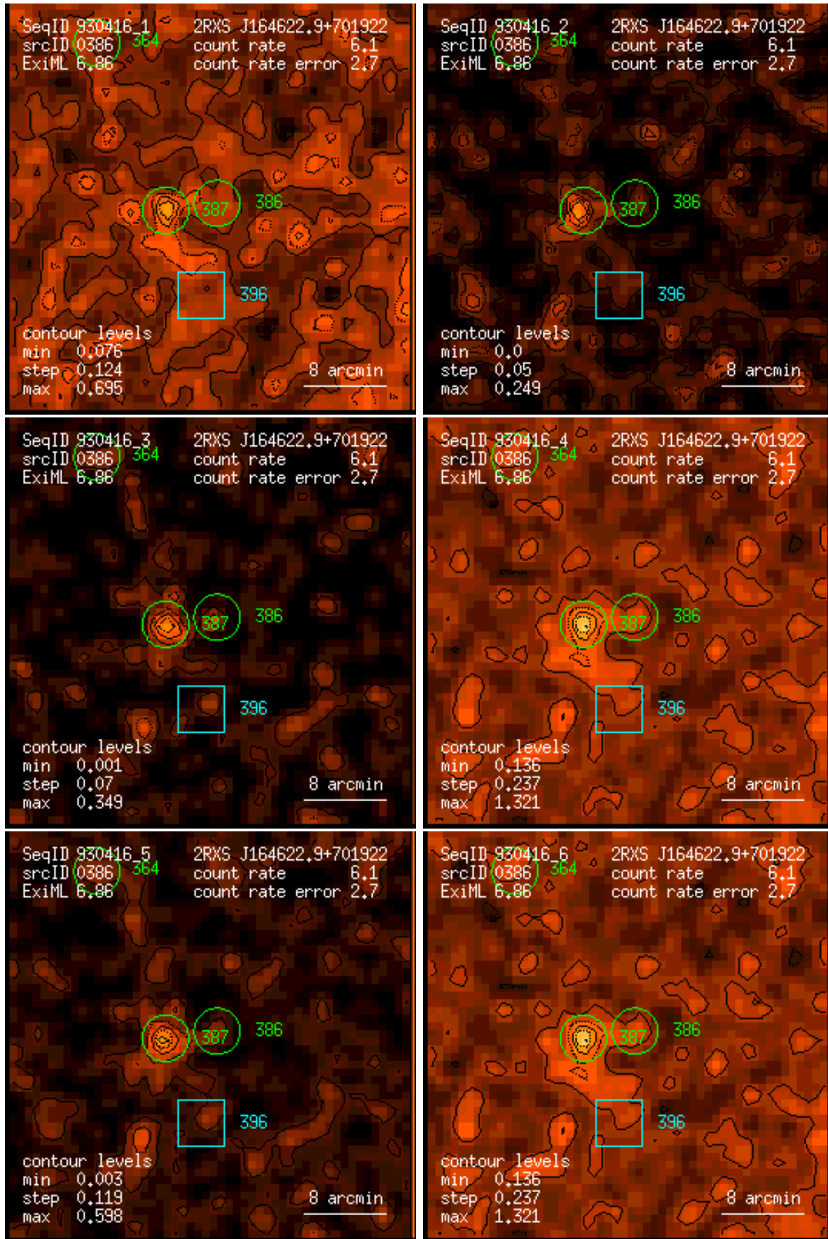
Figure 386: RASS 930416: detection 0386: band rate images, Gaussian filter: (1) PSPC channels 11 – 41, (2) 52 – 90, (3) 91 – 201, (4) 11 – 235, (5) 52 – 201, (6) 11 – 201. Broad band rates in counts/ks. Band rate contour levels in counts/ks/arcmin 2 .
