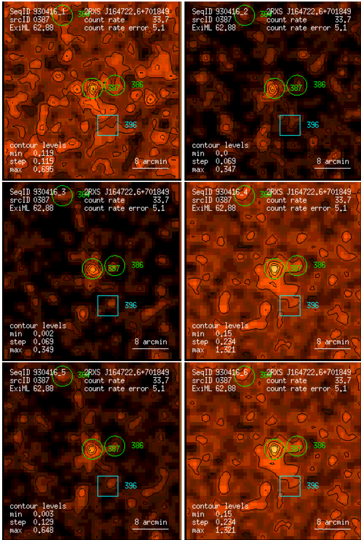
Figure 387: RASS 930416: detection 0387: band rate images, Gaussian filter: (1) PSPC channels 11 – 41, (2) 52 – 90, (3) 91 – 201, (4) 11 – 235, (5) 52 – 201, (6) 11 – 201. Broad band rates in counts/ks. Band rate contour levels in counts/ks/arcmin 2 .
