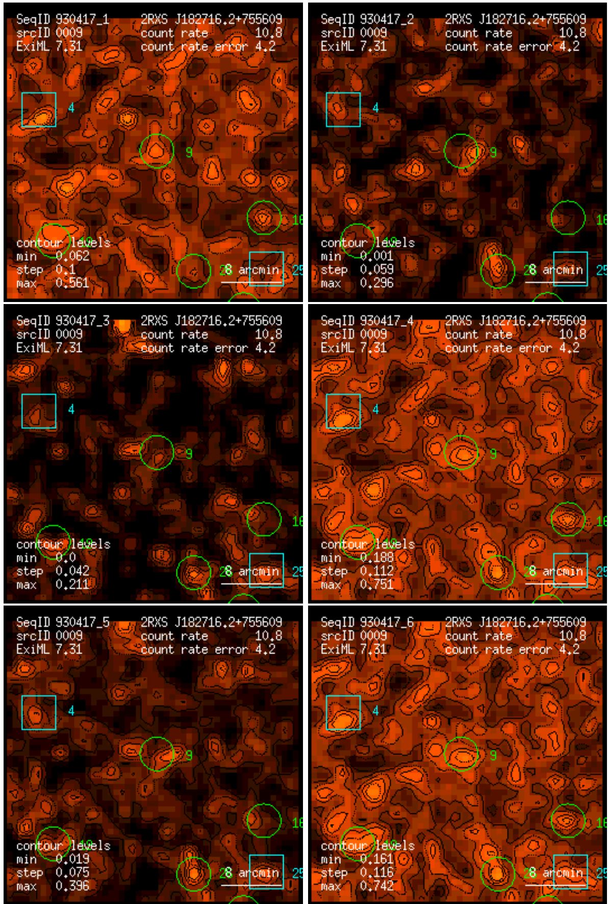
Figure 9: RASS 930417: detection 0009: band rate images, Gaussian filter: (1) PSPC channels 11 – 41, (2) 52 – 90, (3) 91 – 201, (4) 11 – 235, (5) 52 – 201, (6) 11 – 201. Broad band rates in counts/ks. Band rate contour levels in counts/ks/arcmin 2 .
