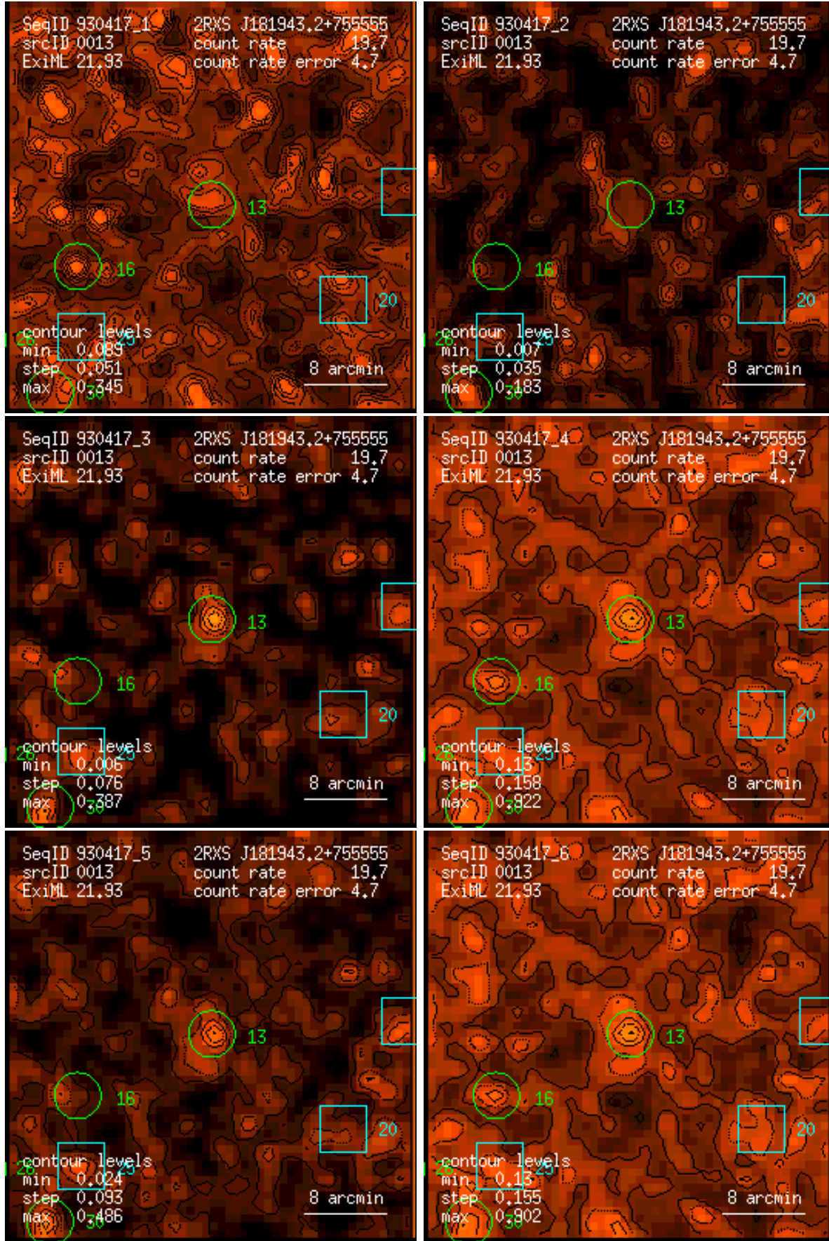
Figure 13: RASS 930417: detection 0013: band rate images, Gaussian filter: (1) PSPC channels 11 – 41, (2) 52 – 90, (3) 91 – 201, (4) 11 – 235, (5) 52 – 201, (6) 11 – 201. Broad band rates in counts/ks. Band rate contour levels in counts/ks/arcmin 2 .
