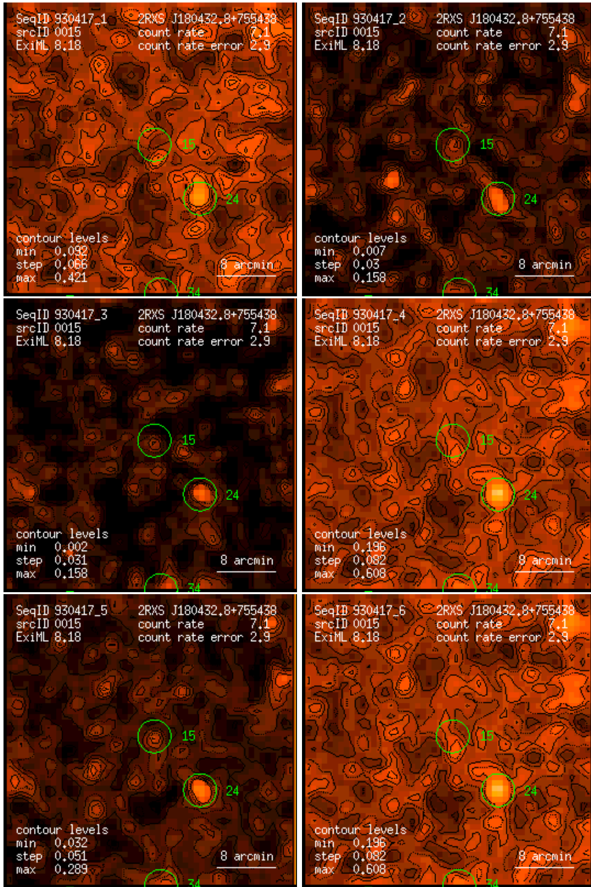
Figure 15: RASS 930417: detection 0015: band rate images, Gaussian filter: (1) PSPC channels 11 – 41, (2) 52 – 90, (3) 91 – 201, (4) 11 – 235, (5) 52 – 201, (6) 11 – 201. Broad band rates in counts/ks. Band rate contour levels in counts/ks/arcmin 2 .
