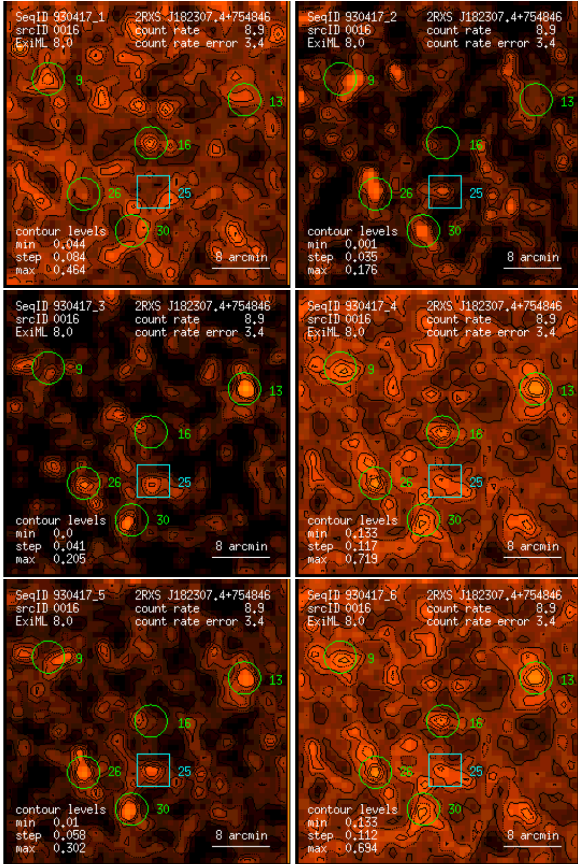
Figure 16: RASS 930417: detection 0016: band rate images, Gaussian filter: (1) PSPC channels 11 – 41, (2) 52 – 90, (3) 91 – 201, (4) 11 – 235, (5) 52 – 201, (6) 11 – 201. Broad band rates in counts/ks. Band rate contour levels in counts/ks/arcmin 2 .
