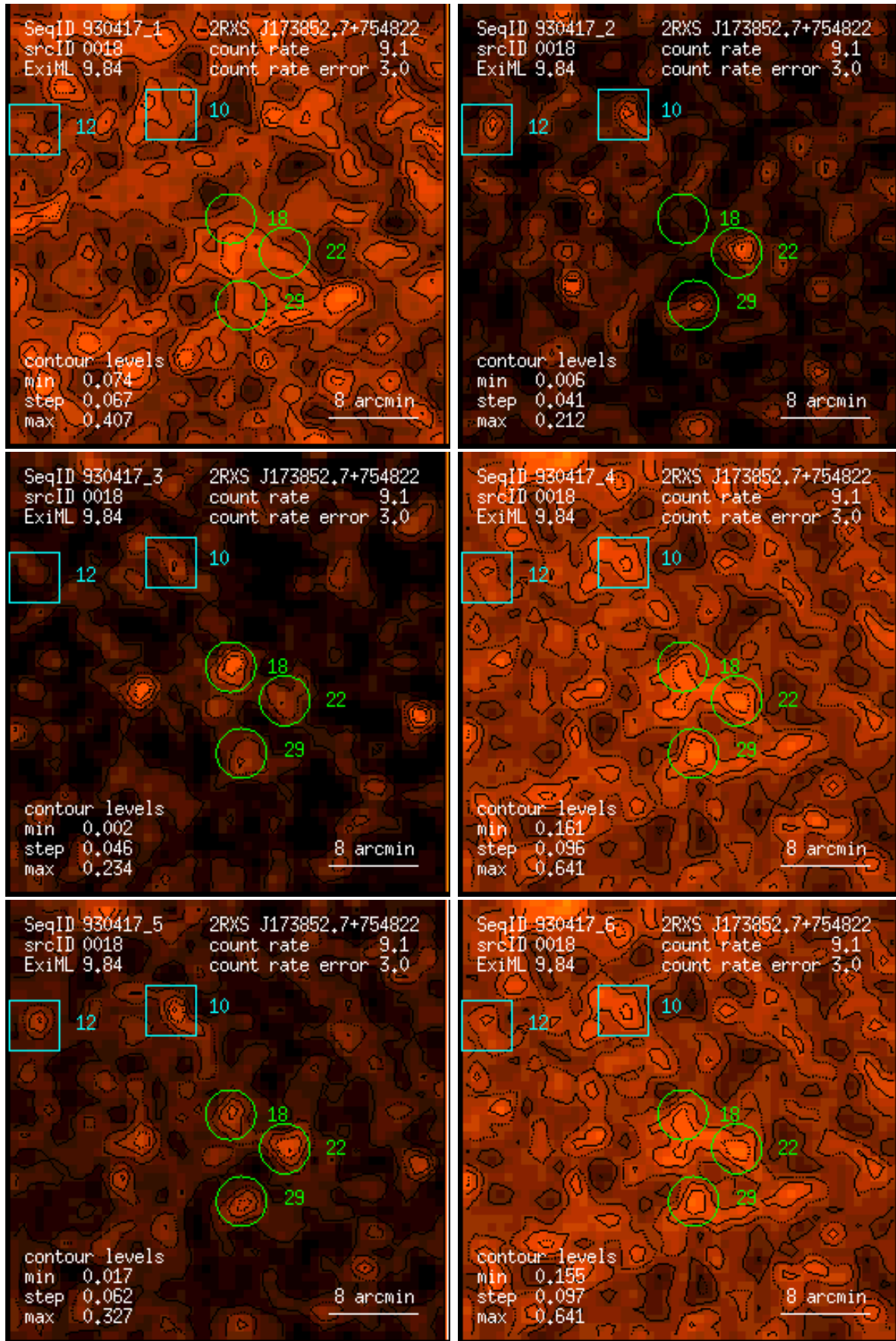
Figure 18: RASS 930417: detection 0018: band rate images, Gaussian filter: (1) PSPC channels 11 – 41, (2) 52 – 90, (3) 91 – 201, (4) 11 – 235, (5) 52 – 201, (6) 11 – 201. Broad band rates in counts/ks. Band rate contour levels in counts/ks/arcmin 2 .
