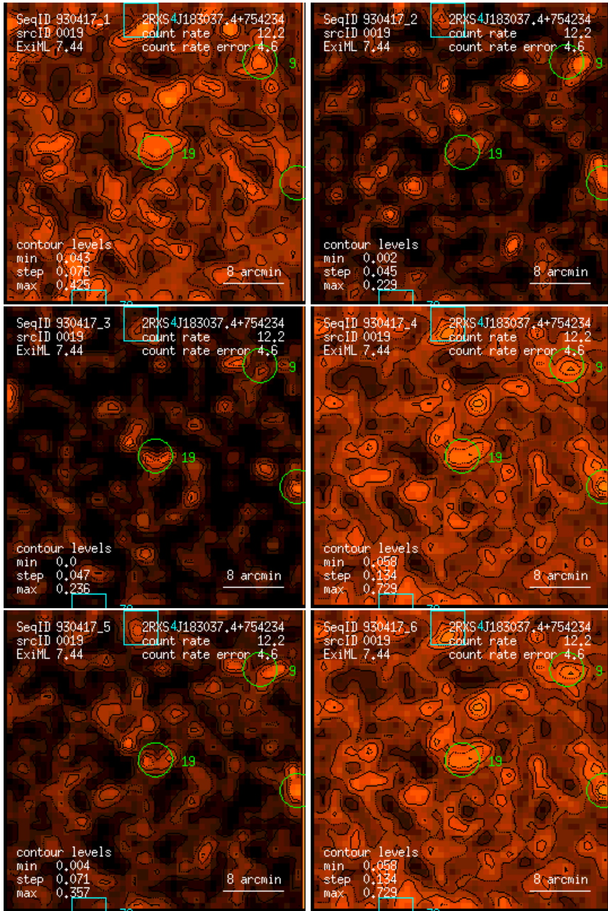
Figure 19: RASS 930417: detection 0019: band rate images, Gaussian filter: (1) PSPC channels 11 – 41, (2) 52 – 90, (3) 91 – 201, (4) 11 – 235, (5) 52 – 201, (6) 11 – 201. Broad band rates in counts/ks. Band rate contour levels in counts/ks/arcmin 2 .
