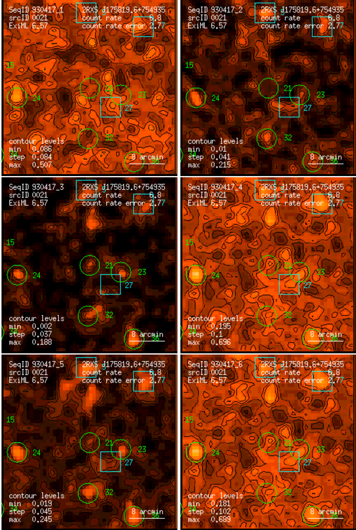
Figure 21: RASS 930417: detection 0021: band rate images, Gaussian filter: (1) PSPC channels 11 – 41, (2) 52 – 90, (3) 91 – 201, (4) 11 – 235, (5) 52 – 201, (6) 11 – 201. Broad band rates in counts/ks. Band rate contour levels in counts/ks/arcmin 2 .
