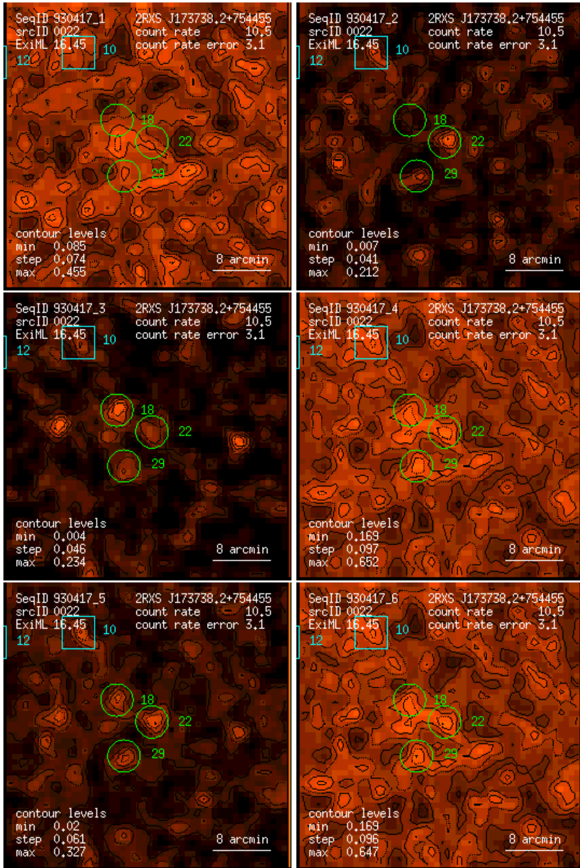
Figure 22: RASS 930417: detection 0022: band rate images, Gaussian filter: (1) PSPC channels 11 – 41, (2) 52 – 90, (3) 91 – 201, (4) 11 – 235, (5) 52 – 201, (6) 11 – 201. Broad band rates in counts/ks. Band rate contour levels in counts/ks/arcmin 2 .
