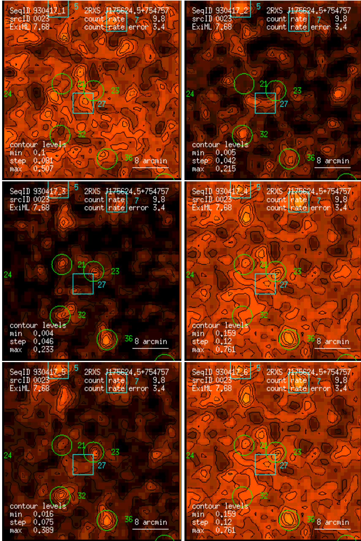
Figure 23: RASS 930417: detection 0023: band rate images, Gaussian filter: (1) PSPC channels 11 – 41, (2) 52 – 90, (3) 91 – 201, (4) 11 – 235, (5) 52 – 201, (6) 11 – 201. Broad band rates in counts/ks. Band rate contour levels in counts/ks/arcmin 2 .
