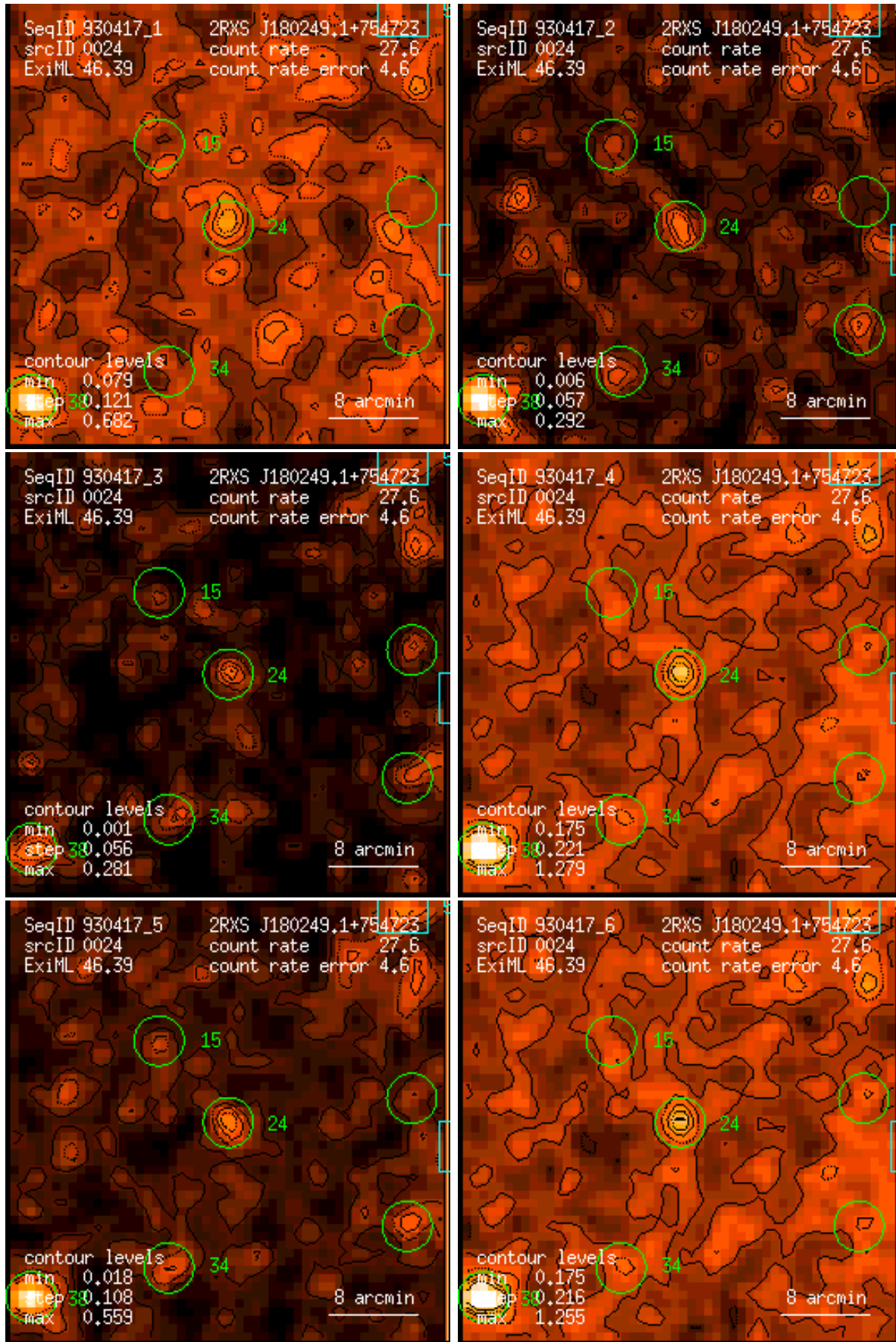
Figure 24: RASS 930417: detection 0024: band rate images, Gaussian filter: (1) PSPC channels 11 – 41, (2) 52 – 90, (3) 91 – 201, (4) 11 – 235, (5) 52 – 201, (6) 11 – 201. Broad band rates in counts/ks. Band rate contour levels in counts/ks/arcmin 2 .
