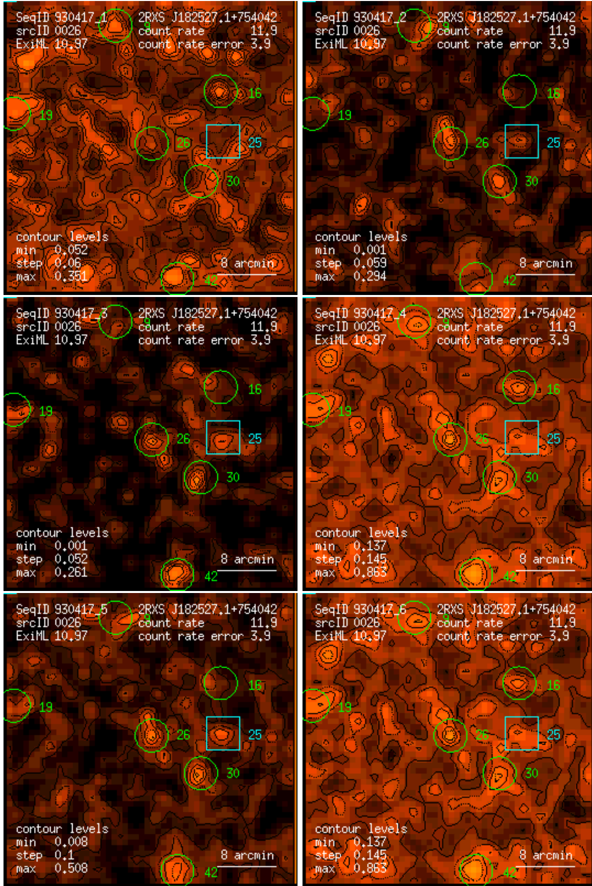
Figure 26: RASS 930417: detection 0026: band rate images, Gaussian filter: (1) PSPC channels 11 – 41, (2) 52 – 90, (3) 91 – 201, (4) 11 – 235, (5) 52 – 201, (6) 11 – 201. Broad band rates in counts/ks. Band rate contour levels in counts/ks/arcmin 2 .
