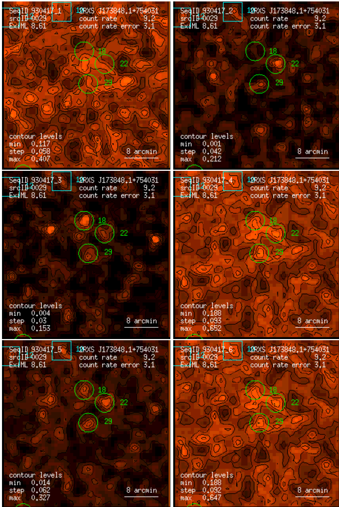
Figure 29: RASS 930417: detection 0029: band rate images, Gaussian filter: (1) PSPC channels 11 – 41, (2) 52 – 90, (3) 91 – 201, (4) 11 – 235, (5) 52 – 201, (6) 11 – 201. Broad band rates in counts/ks. Band rate contour levels in counts/ks/arcmin 2 .
