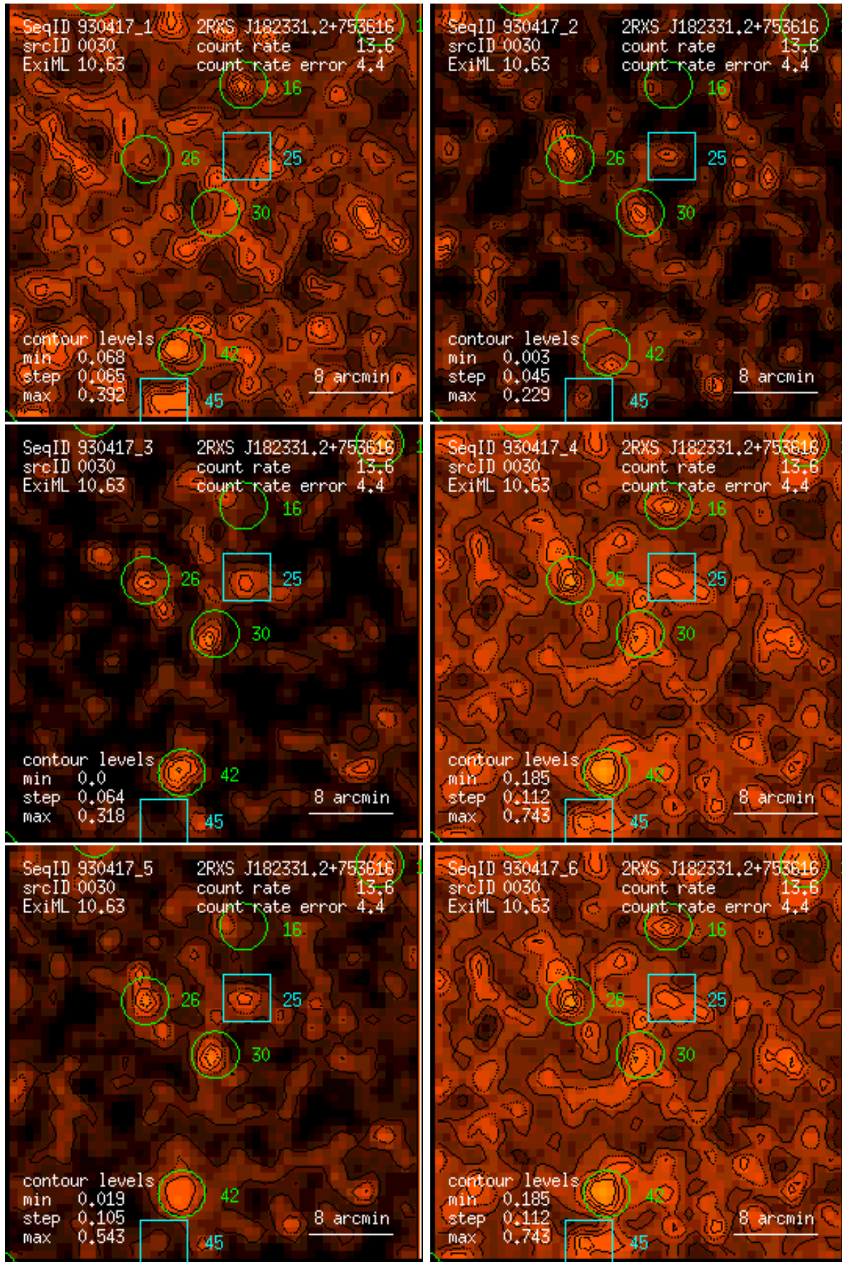
Figure 30: RASS 930417: detection 0030: band rate images, Gaussian filter: (1) PSPC channels 11 – 41, (2) 52 – 90, (3) 91 – 201, (4) 11 – 235, (5) 52 – 201, (6) 11 – 201. Broad band rates in counts/ks. Band rate contour levels in counts/ks/arcmin 2 .
