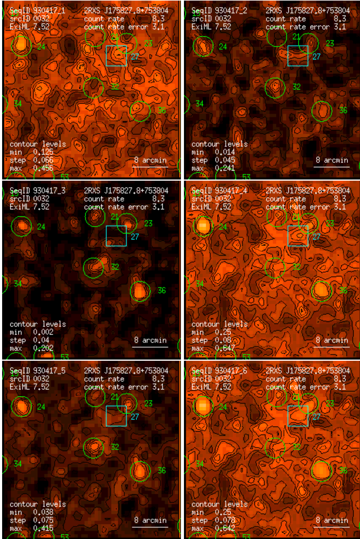
Figure 32: RASS 930417: detection 0032: band rate images, Gaussian filter: (1) PSPC channels 11 – 41, (2) 52 – 90, (3) 91 – 201, (4) 11 – 235, (5) 52 – 201, (6) 11 – 201. Broad band rates in counts/ks. Band rate contour levels in counts/ks/arcmin 2 .
