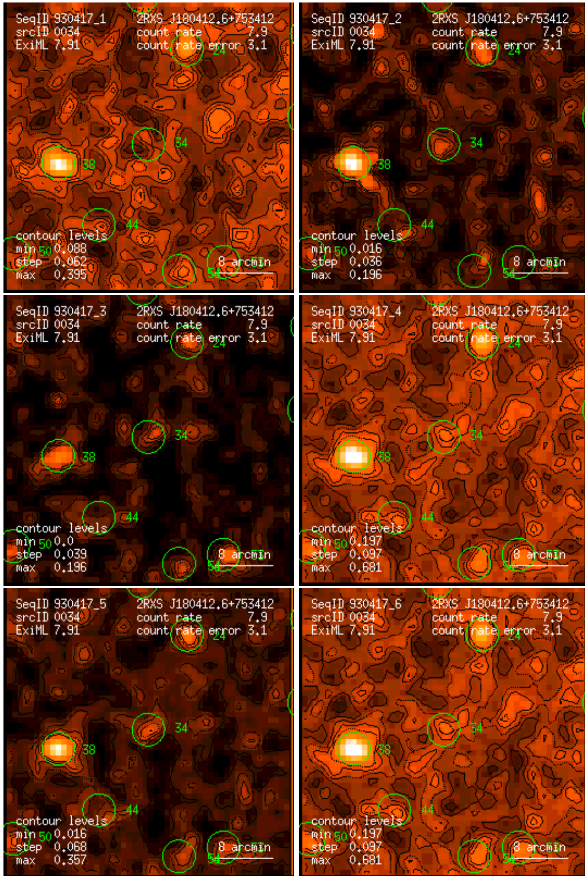
Figure 34: RASS 930417: detection 0034: band rate images, Gaussian filter: (1) PSPC channels 11 – 41, (2) 52 – 90, (3) 91 – 201, (4) 11 – 235, (5) 52 – 201, (6) 11 – 201. Broad band rates in counts/ks. Band rate contour levels in counts/ks/arcmin 2 .
