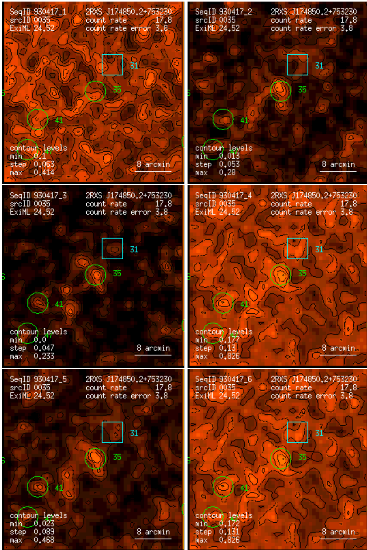
Figure 35: RASS 930417: detection 0035: band rate images, Gaussian filter: (1) PSPC channels 11 – 41, (2) 52 – 90, (3) 91 – 201, (4) 11 – 235, (5) 52 – 201, (6) 11 – 201. Broad band rates in counts/ks. Band rate contour levels in counts/ks/arcmin 2 .
