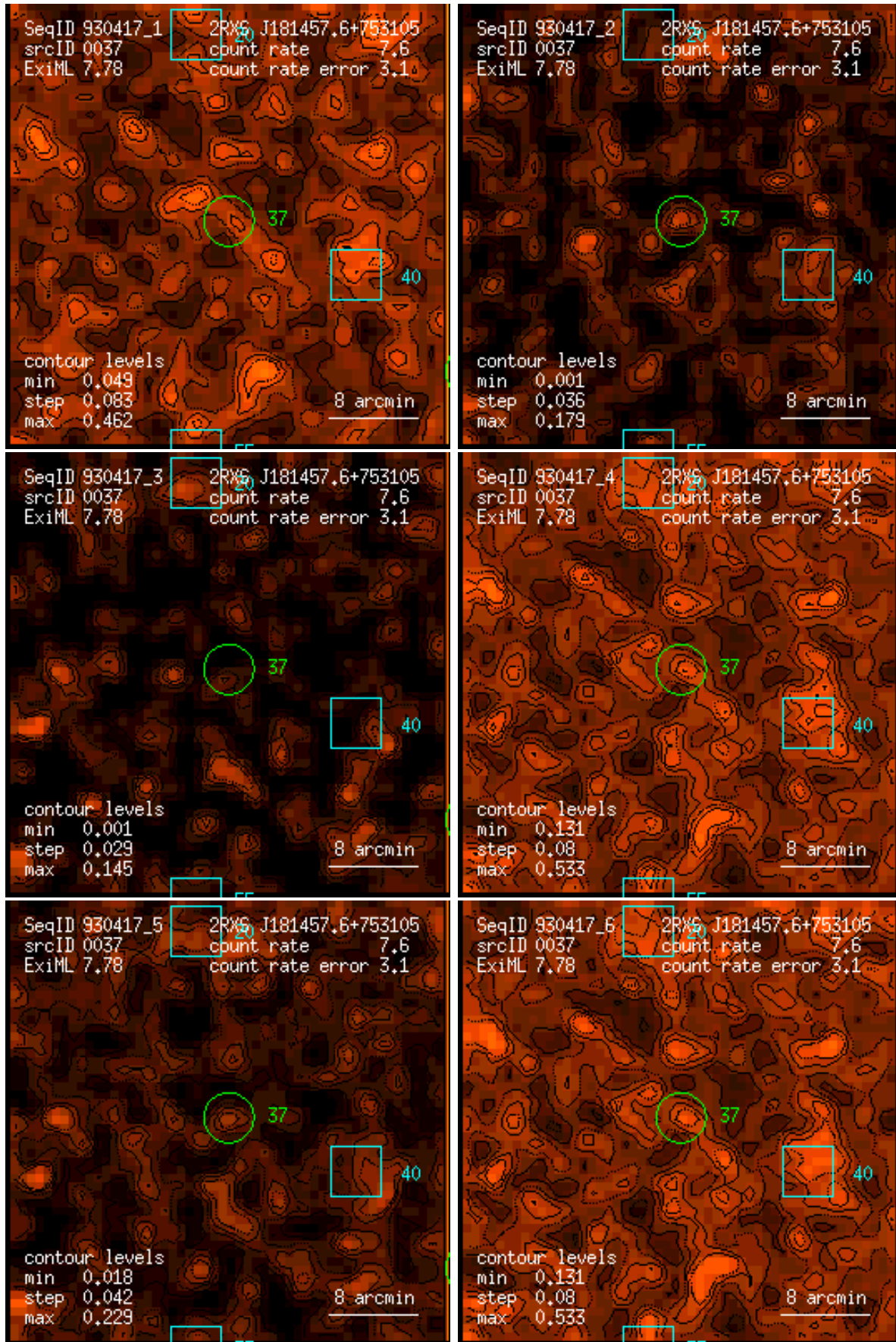
Figure 37: RASS 930417: detection 0037: band rate images, Gaussian filter: (1) PSPC channels 11 – 41, (2) 52 – 90, (3) 91 – 201, (4) 11 – 235, (5) 52 – 201, (6) 11 – 201. Broad band rates in counts/ks. Band rate contour levels in counts/ks/arcmin 2 .
