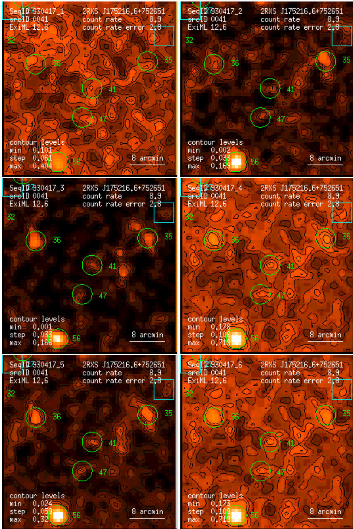
Figure 41: RASS 930417: detection 0041: band rate images, Gaussian filter: (1) PSPC channels 11 – 41, (2) 52 – 90, (3) 91 – 201, (4) 11 – 235, (5) 52 – 201, (6) 11 – 201. Broad band rates in counts/ks. Band rate contour levels in counts/ks/arcmin 2 .
