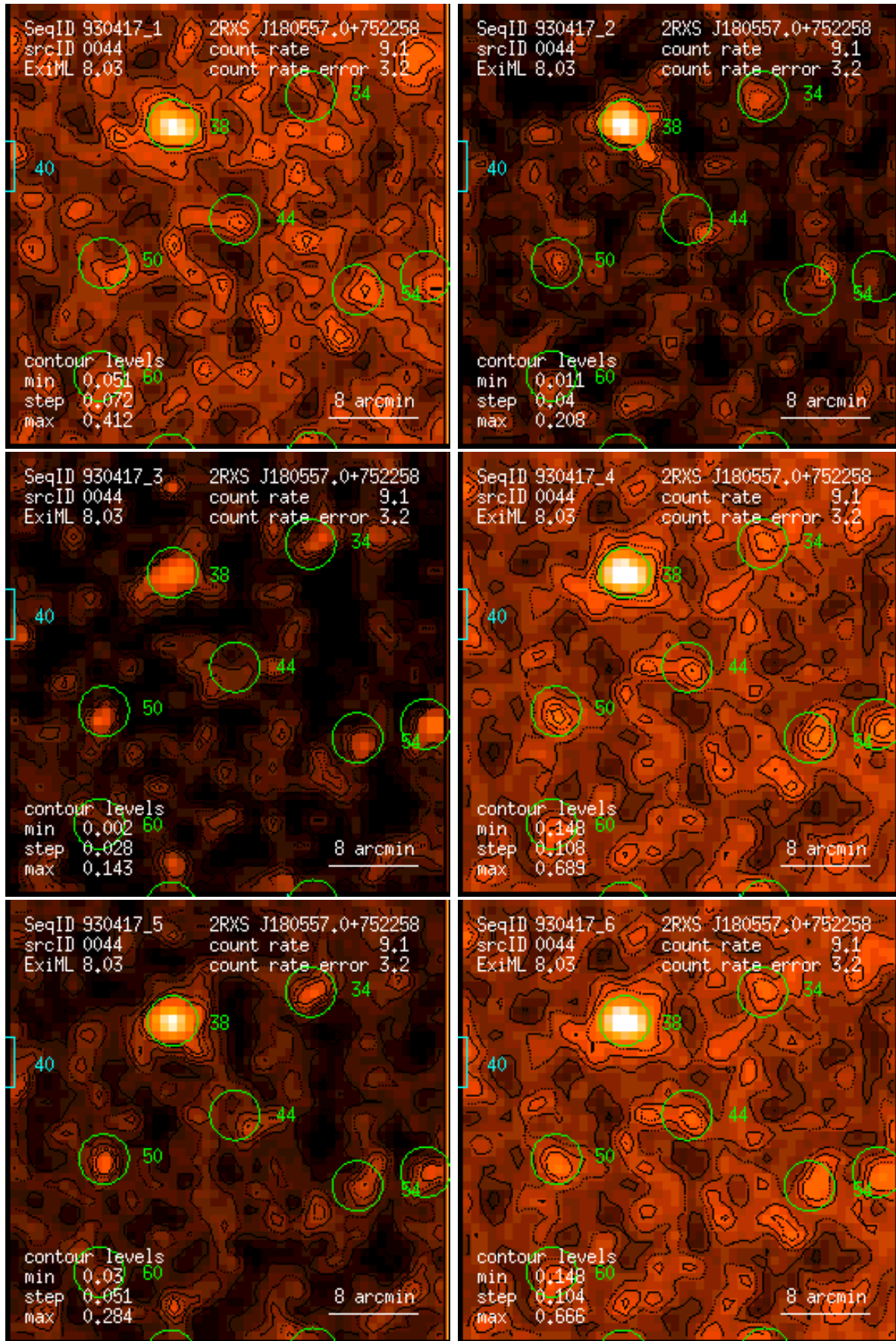
Figure 44: RASS 930417: detection 0044: band rate images, Gaussian filter: (1) PSPC channels 11 – 41, (2) 52 – 90, (3) 91 – 201, (4) 11 – 235, (5) 52 – 201, (6) 11 – 201. Broad band rates in counts/ks. Band rate contour levels in counts/ks/arcmin 2 .
