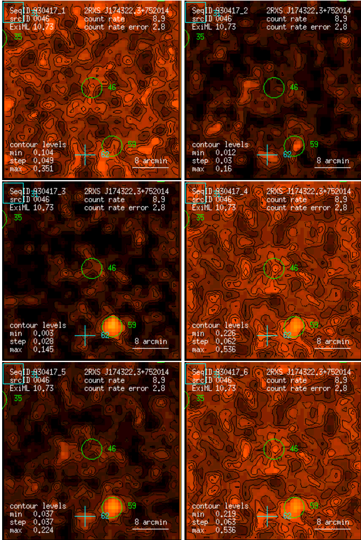
Figure 46: RASS 930417: detection 0046: band rate images, Gaussian filter: (1) PSPC channels 11 – 41, (2) 52 – 90, (3) 91 – 201, (4) 11 – 235, (5) 52 – 201, (6) 11 – 201. Broad band rates in counts/ks. Band rate contour levels in counts/ks/arcmin 2 .
