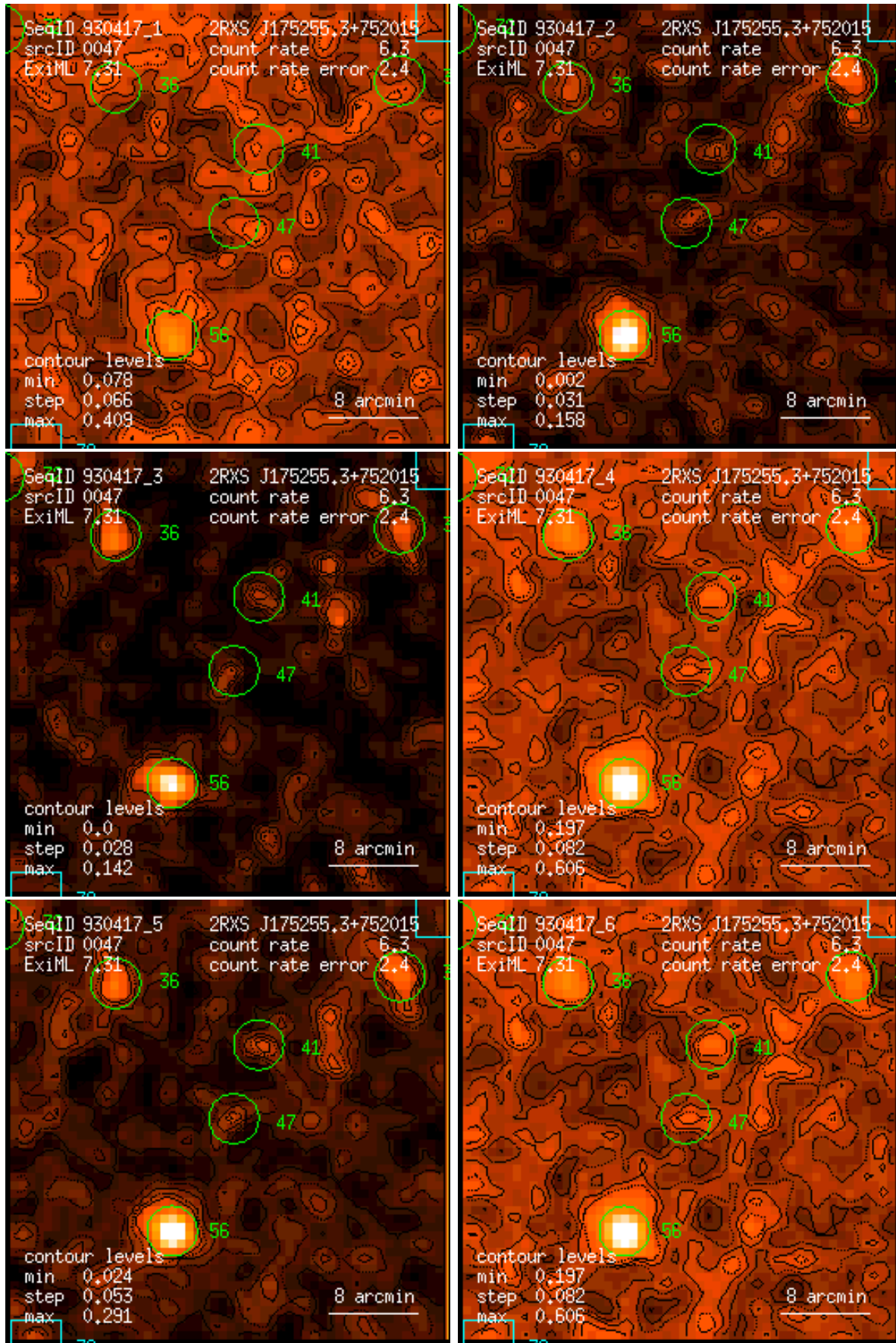
Figure 47: RASS 930417: detection 0047: band rate images, Gaussian filter: (1) PSPC channels 11 – 41, (2) 52 – 90, (3) 91 – 201, (4) 11 – 235, (5) 52 – 201, (6) 11 – 201. Broad band rates in counts/ks. Band rate contour levels in counts/ks/arcmin 2 .
