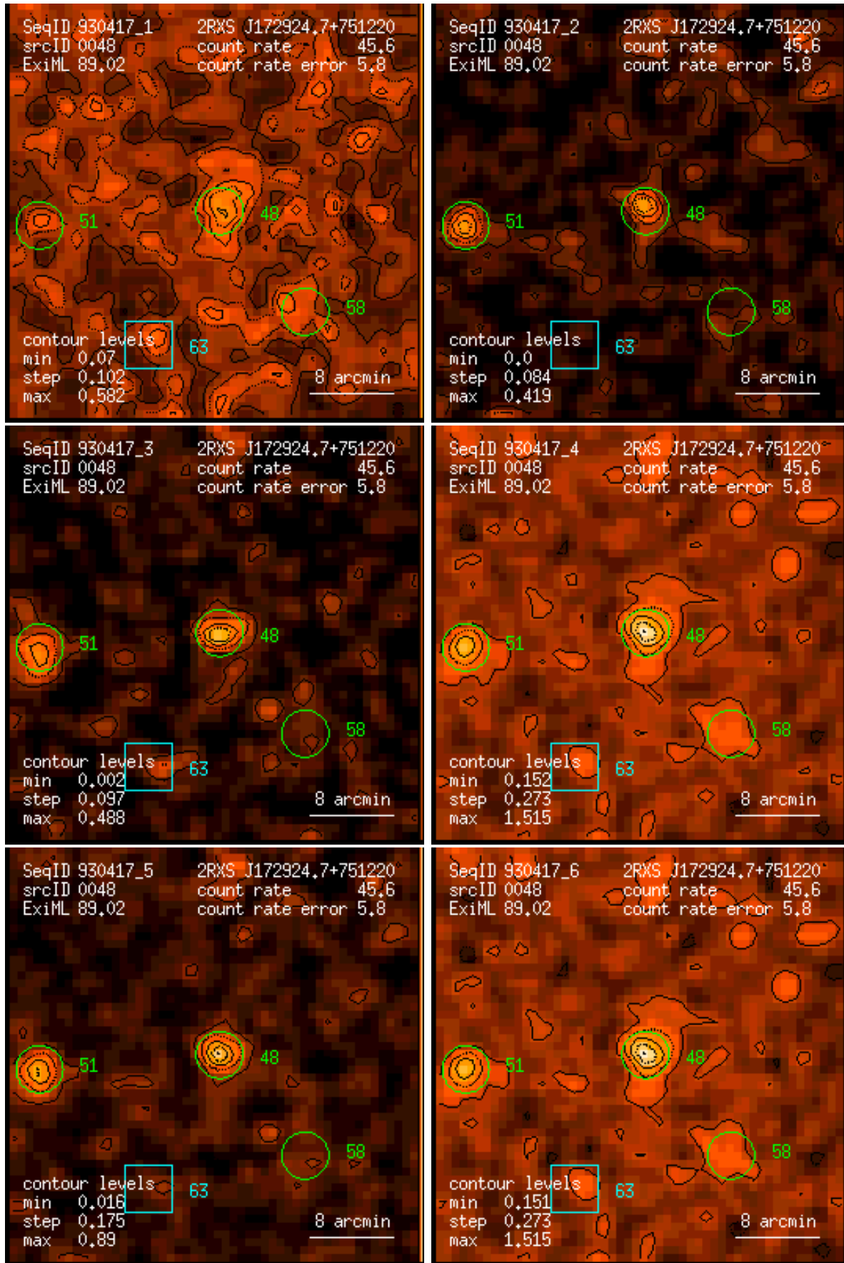
Figure 48: RASS 930417: detection 0048: band rate images, Gaussian filter: (1) PSPC channels 11 – 41, (2) 52 – 90, (3) 91 – 201, (4) 11 – 235, (5) 52 – 201, (6) 11 – 201. Broad band rates in counts/ks. Band rate contour levels in counts/ks/arcmin 2 .
