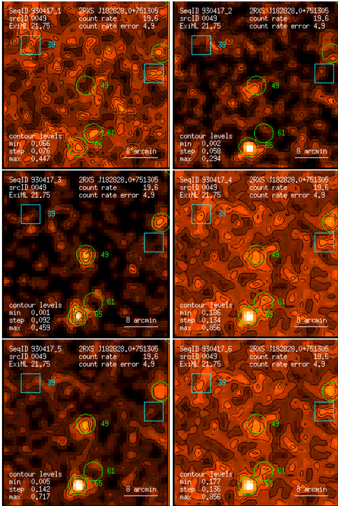
Figure 49: RASS 930417: detection 0049: band rate images, Gaussian filter: (1) PSPC channels 11 – 41, (2) 52 – 90, (3) 91 – 201, (4) 11 – 235, (5) 52 – 201, (6) 11 – 201. Broad band rates in counts/ks. Band rate contour levels in counts/ks/arcmin 2 .
