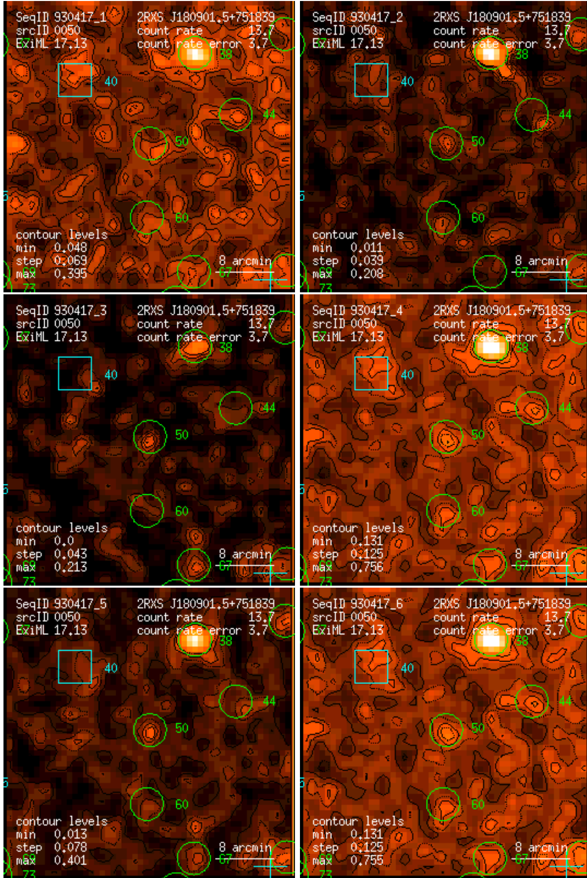
Figure 50: RASS 930417: detection 0050: band rate images, Gaussian filter: (1) PSPC channels 11 – 41, (2) 52 – 90, (3) 91 – 201, (4) 11 – 235, (5) 52 – 201, (6) 11 – 201. Broad band rates in counts/ks. Band rate contour levels in counts/ks/arcmin 2 .
